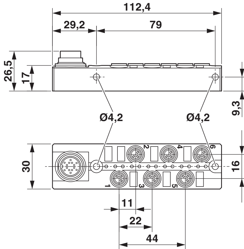
Dimensional drawing
