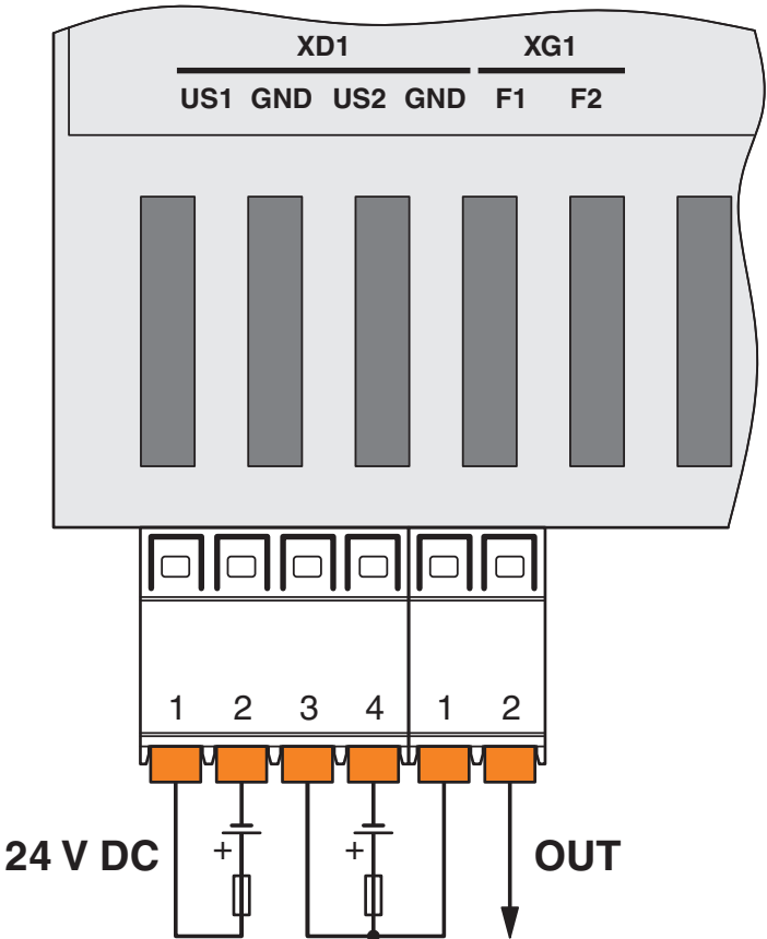
Connection diagram
