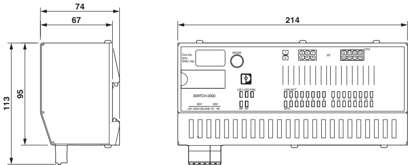
Dimensional drawing
