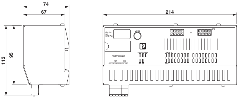
Dimensional drawing
