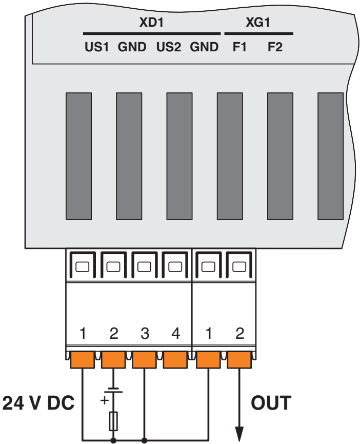
Connection diagram
