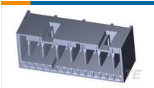
TE Part # 2232043-7 7P, RAST 5 Tab Header, THV
