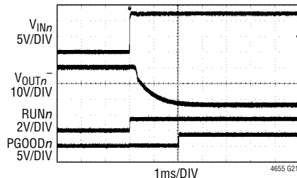
Start-Up, No Load
