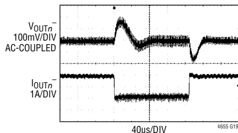
-5V Transient Response, 24V_{IN}
