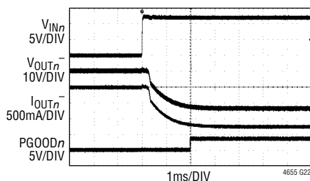
Start-Up, 1.25A Load
