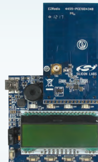
EZRadio® Si4010/Si4355 ONE-WAY AES DEVELOPMENT KIT
