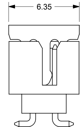
VIEW FOR HEADER WITH CAP
