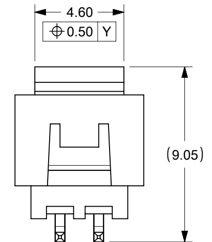
VIEW FOR HEADER WITH CAP
