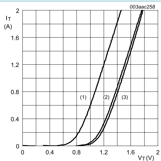
V_o = 1.13 V; R_s = 0.31 \Omega (1) T_j = 125^\circ C ; typical values (2) T_j = 125^\circ C ; maximum values (3) T_j = 25^\circ C ; maximum values Fig. 10. On-state current as a function of on-state voltage
