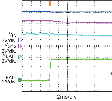
Battery Insertion
