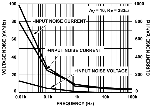
FIGURE 51. INPUT NOISE CHARACTERISTICS
