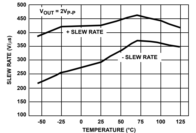
FIGURE 48. SLEW RATE vs TEMPERATURE
