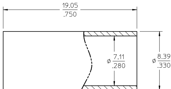
SHRINK TUBE
