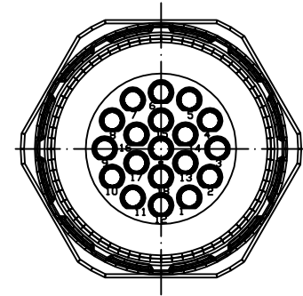
19-Pole (16+3)
