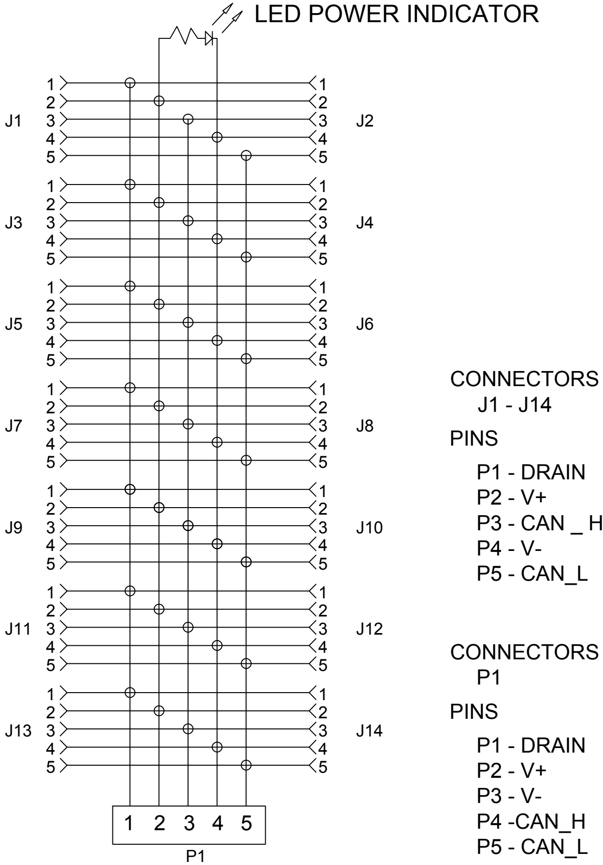
PCR BOARD SCHEMATIC
