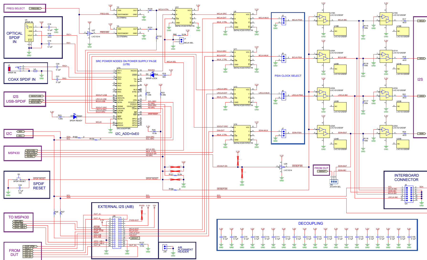
Figure 32. TAS3251EVM Schematics (3 of 5)
