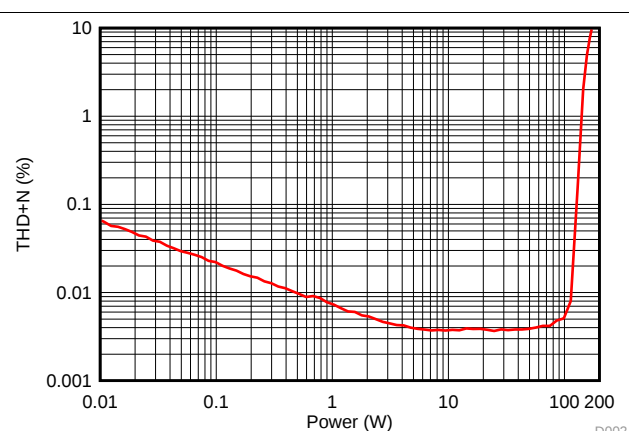
Figure 5. PSIA Input: THD+N vs Power
