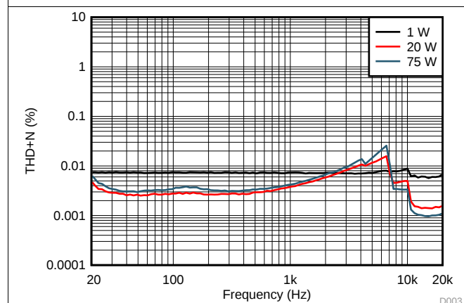
Figure 6. SPDIF Input: THD+N vs Frequency
