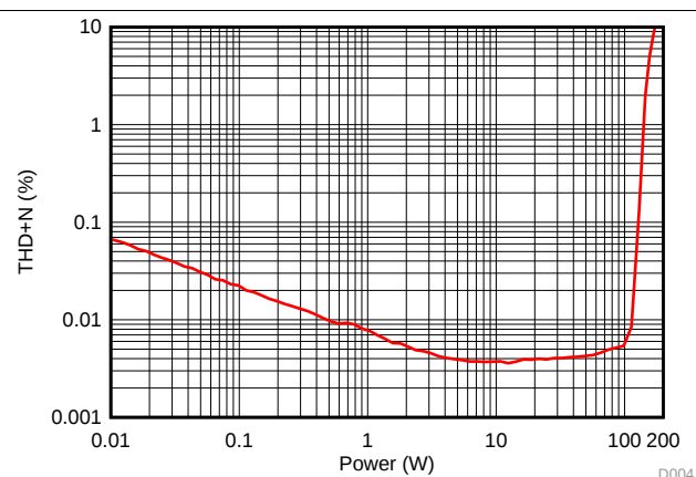
Figure 7. SPDIF Input: THD+N vs Power
