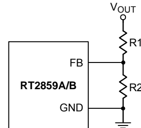
Figure 4. Output Voltage Setting
