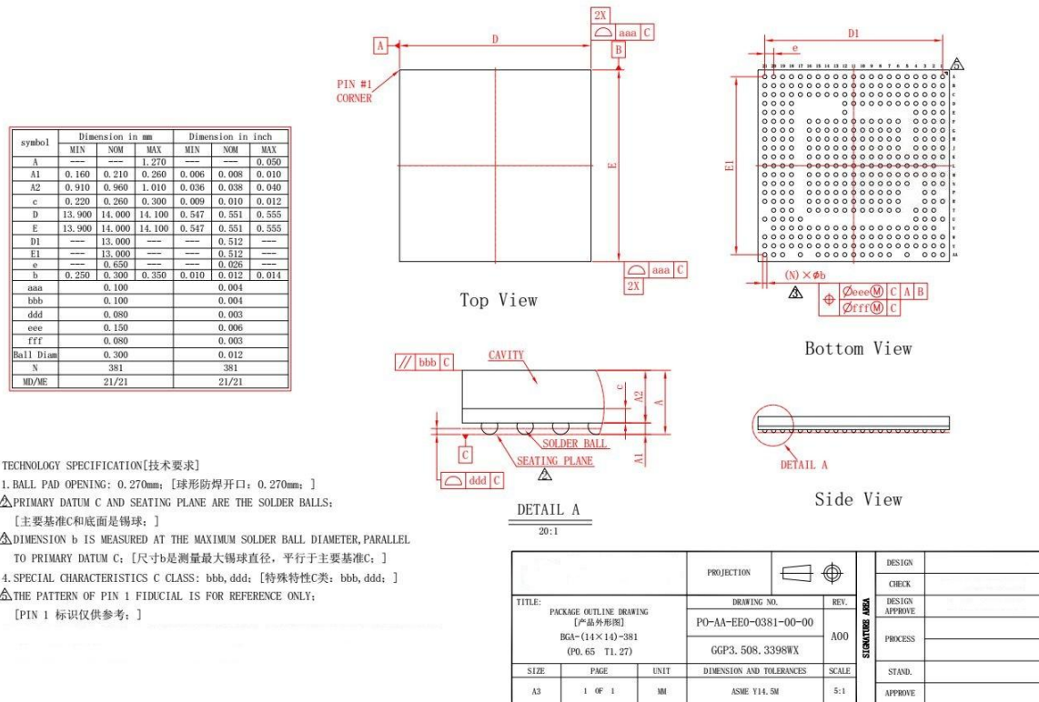
Figure2- 1 T40A package outline drawing
