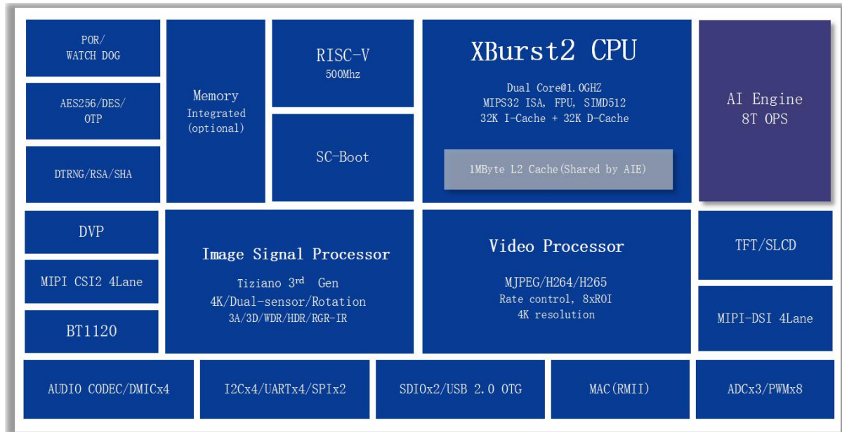
Figure1- 1 T40A Diagram
