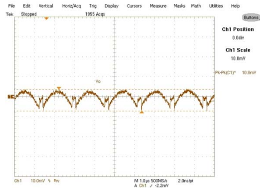
Fig. 10: Output Voltage Ripple, 16A load Ch 1 : V out ,
