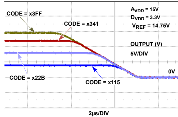
FIGURE 10. OUT1-OUT14 NEGATIVE SLEW RATE (DAC CODE CHANGE)
