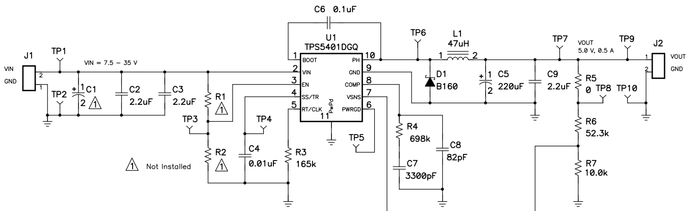
Figure 14. TPS5401EVM-708 Schematic
