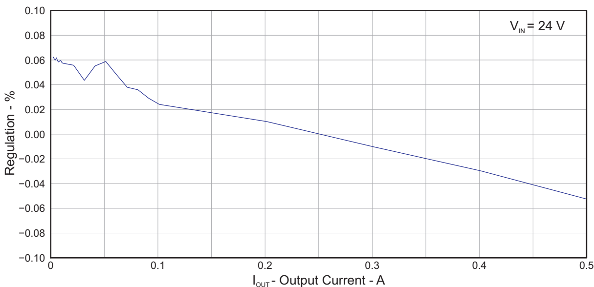
Figure 3. TPS5401EVM-708 Load Regulation
