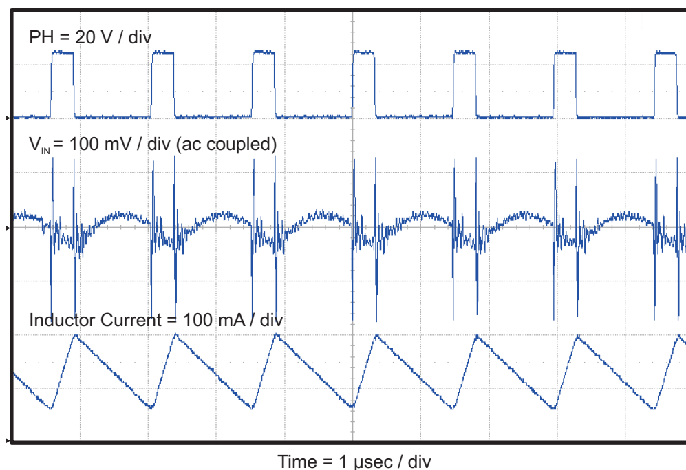
Figure 8. TPS5401EVM-708 Input Ripple
