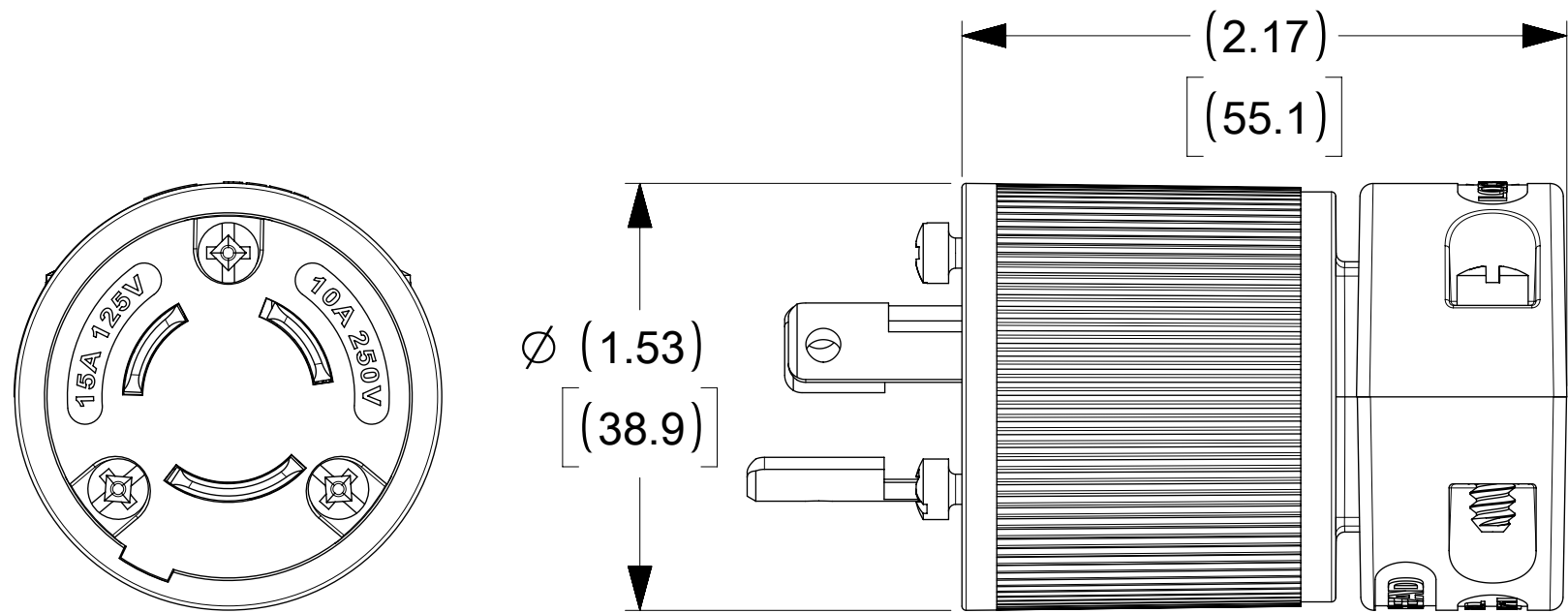
FACE VIEW
