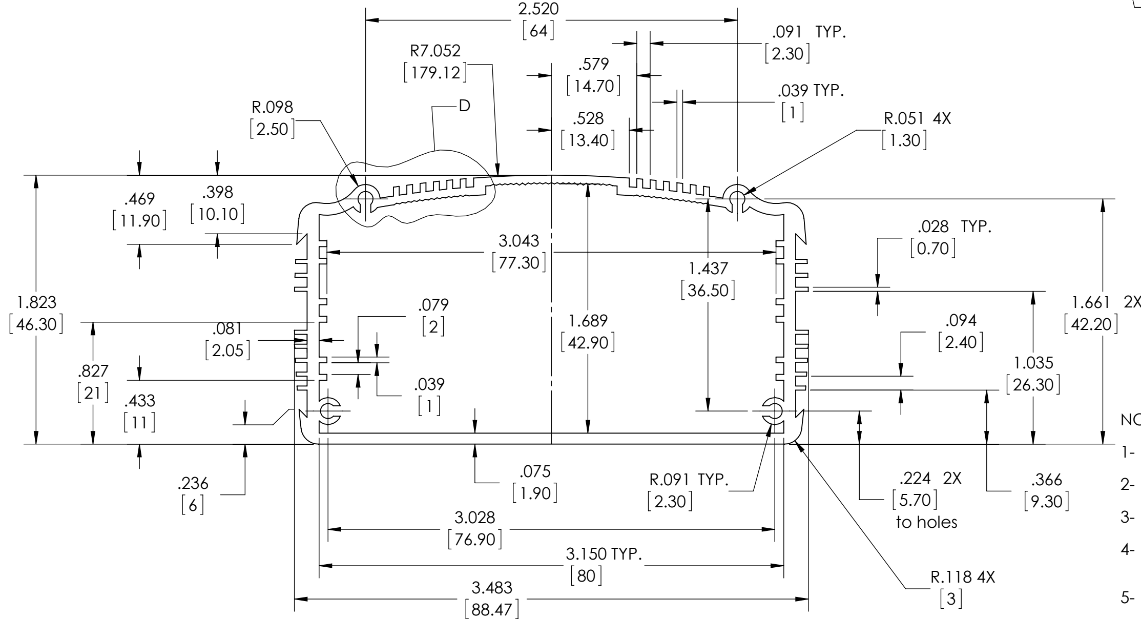
EXTRUSION PROFILE
