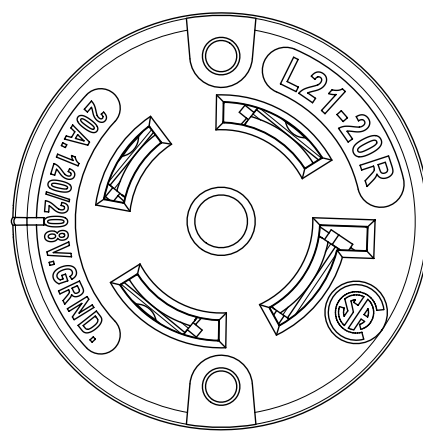
FACE VIEW
