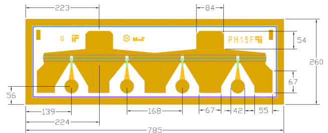
Chip Dimensions: 785 x 260 microns Chip Thickness: 100 microns
