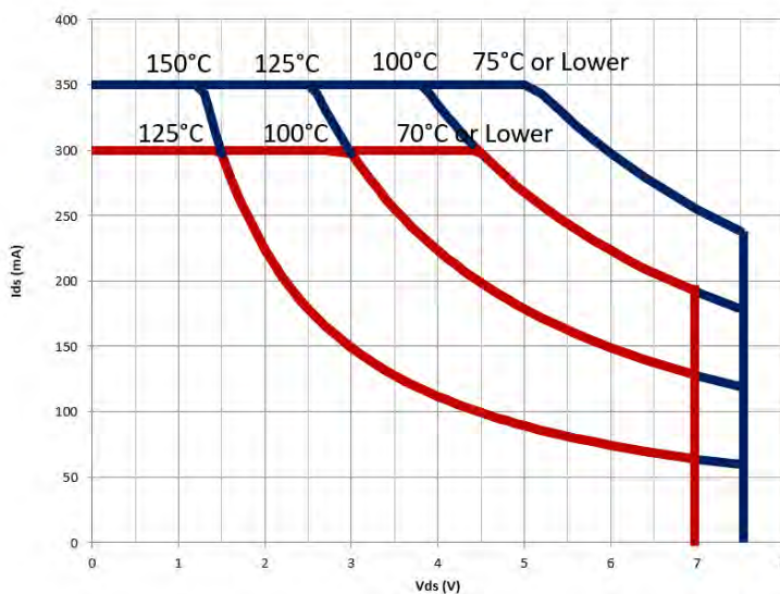
SAFE OPERATING LIMITS vs BACKSIDE TEMPERATURE MwT-PH15F Chip and 71 Pkg
