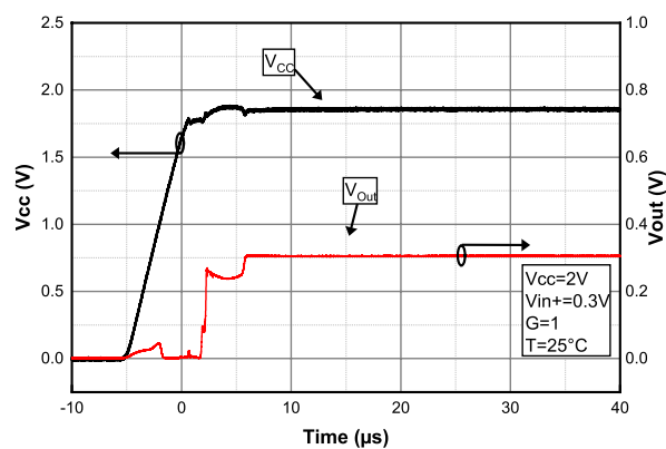
Figure 43. Turn-on time at V_{CC} = 2\text{ V}
