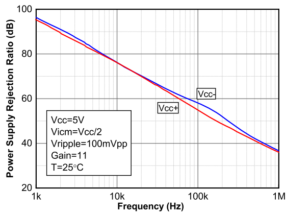
Figure 41. PSRR vs. frequency at V_{CC} = 5\text{ V}
