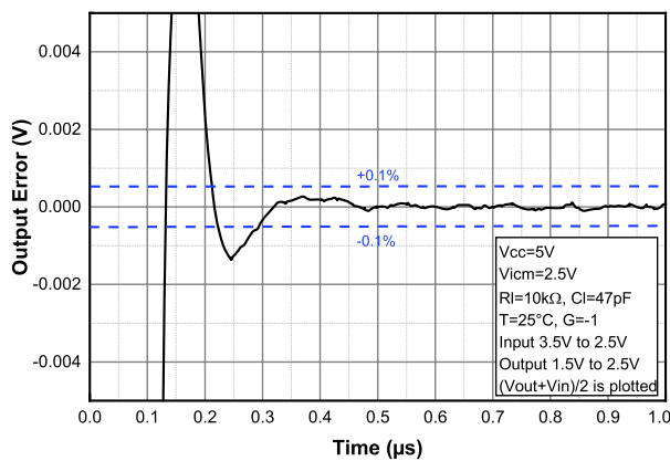
Figure 33. Settling time output low to high at V_{CC} = 5\text{ V}
