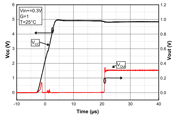
Figure 42. Turn-on time at V_{CC} = 5\text{ V}
