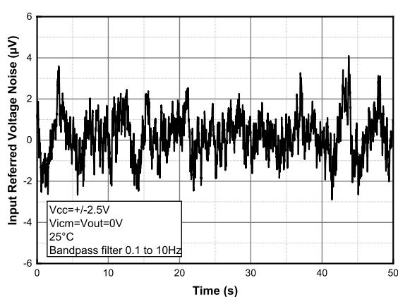
Figure 37. Noise vs. time at V_{CC} = 5\text{ V}
