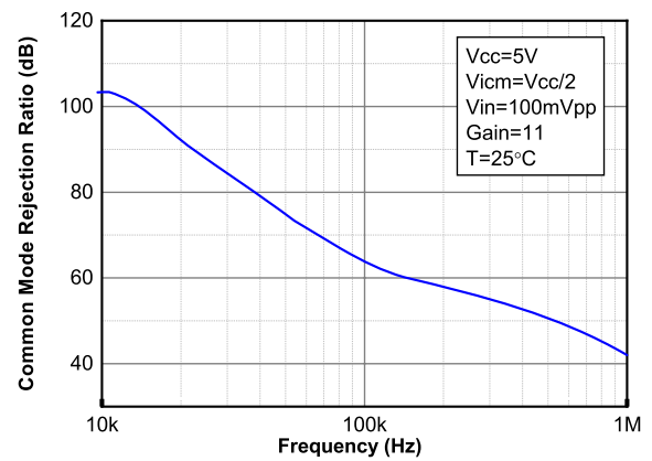
Figure 40. CMRR vs. frequency at V_{CC} = 5\text{ V}
