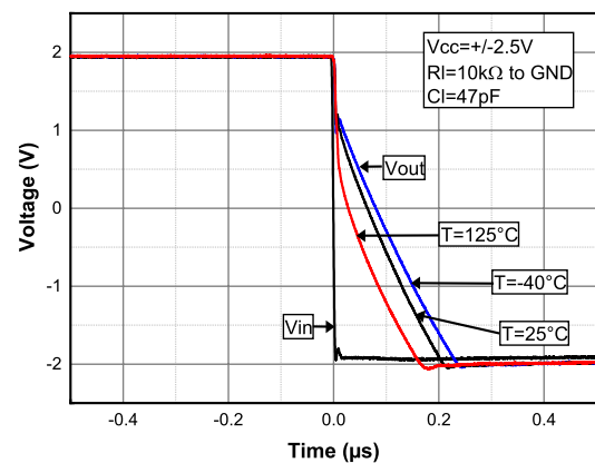
Figure 20. Negative slew rate at V_{CC} = 5\text{ V}
