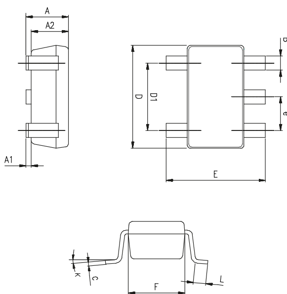
Figure 50. SOT23-5 package outline
