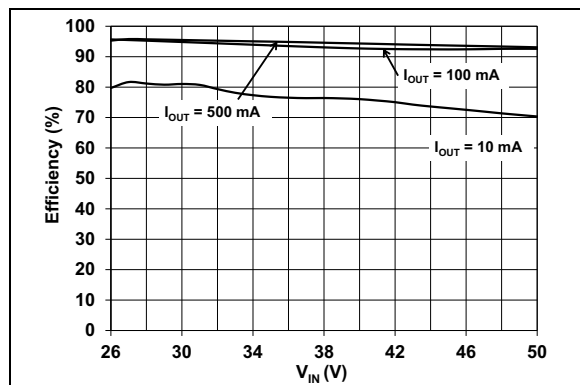
FIGURE 2-8: 24V V_{OUT} Efficiency vs. V_{IN} .
