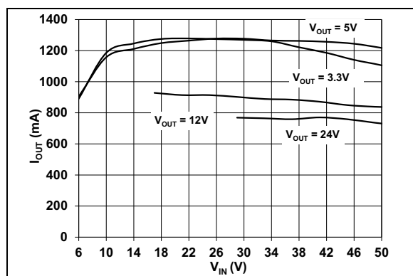
FIGURE 2-9: Max I_{OUT} vs. V_{IN} .
