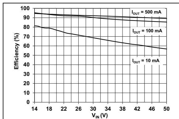
FIGURE 2-7: 12V V_{OUT} Efficiency vs. V_{IN} .
