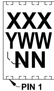
8-Lead TDFN (2x3x0.75 mm)
