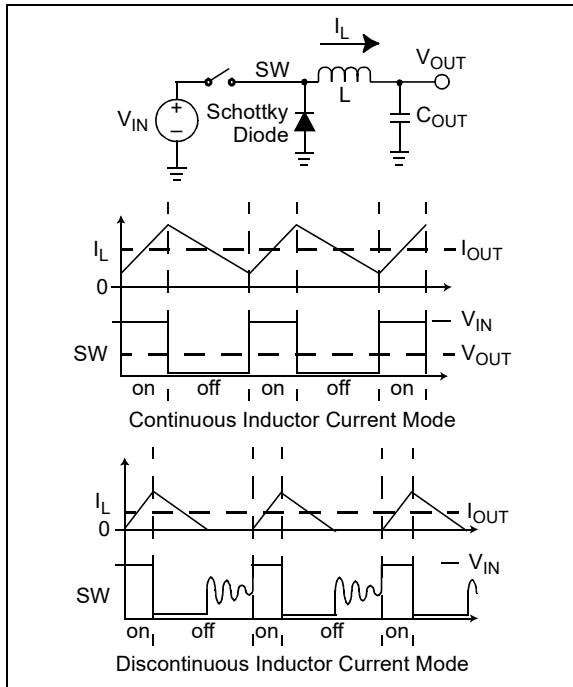
FIGURE 4-2: Step-Down Converter.
