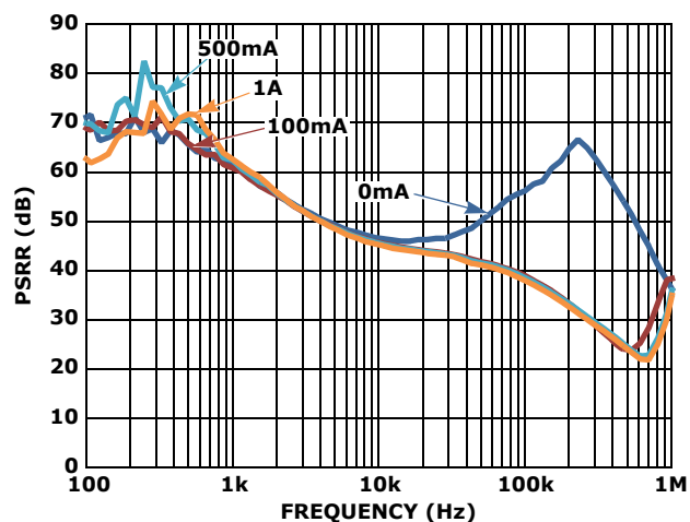
FIGURE 12. V_{IN} = 2.5V , V_{OUT} = 1.2V , C_{OUT} = 22\mu F , C_{PB} = 120pF
