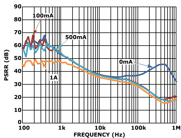
FIGURE 17. V_{IN} = 3.7V , V_{OUT} = 3.3V , C_{OUT} = 10\mu F , C_{PB} = 100pF
