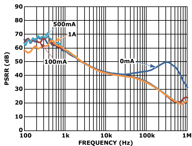
FIGURE 15. V_{IN} = 2.5V , V_{OUT} = 1.8V , C_{OUT} = 10\mu F , C_{PB} = 82pF
