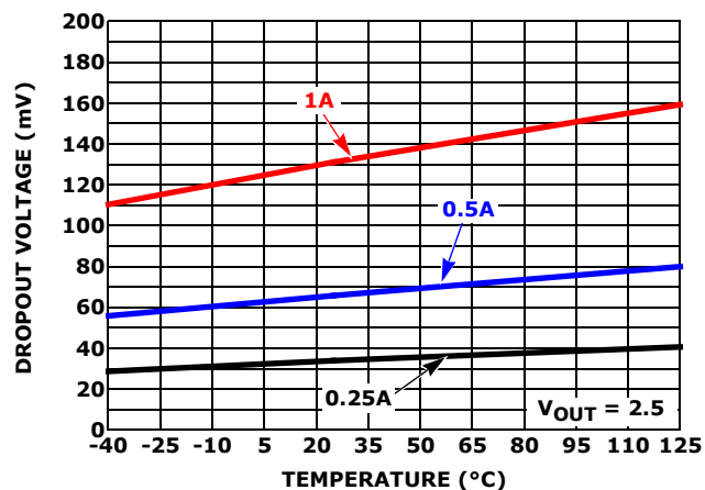
FIGURE 8. DROPOUT AT 1A vs TEMPERATURE
