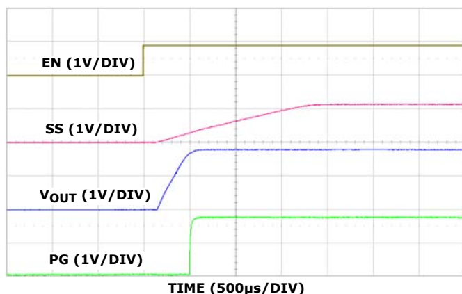
FIGURE 3. START-UP WAVEFORMS
