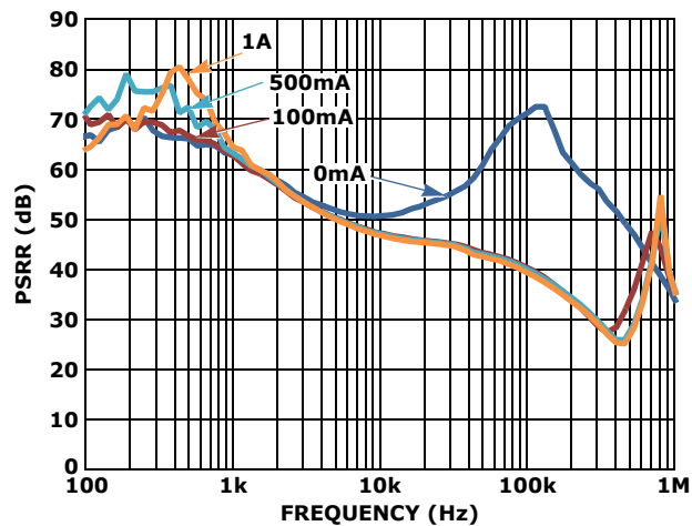
FIGURE 10. V_{IN} = 2.5V , V_{OUT} = 1.0V , C_{OUT} = 47\mu F , C_{PB} = 220pF
