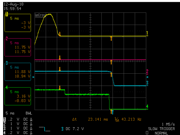
Figure 4: DS460S-3-002 Hold-up time – Vin = 264Vac / 47Hz / 0° Full Load: Vo = 36A, VSB = 2.3A Ch 1: AC Mains Ch 2: VSB Ch 3: Vo Ch 4: PSOK
