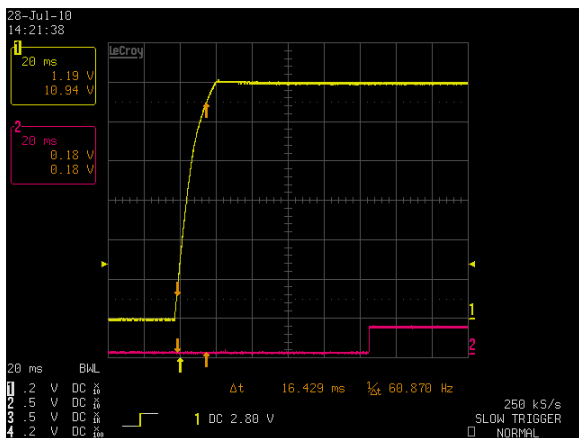
Figure 5: DS460S-3-002 Output Voltage Startup Characteristic – Vin = 90Vac Full Load: Vo = 36A, VSB = 2.3A Ch 1: Vo Ch 2: PSOK
