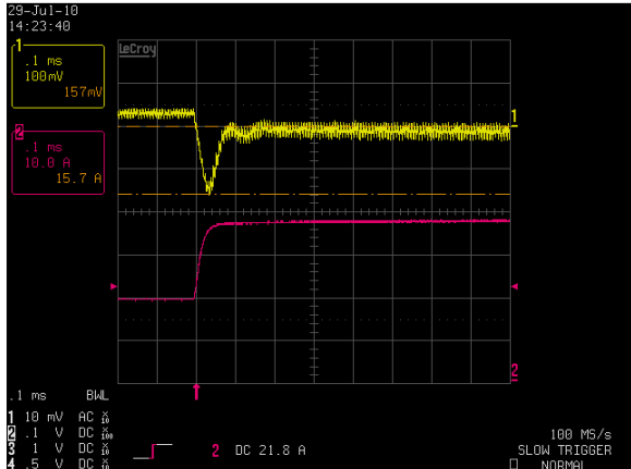
Figure 7: DS460S-3-002 Transient Response – Vo Deviation (low to high) 50% to 100% load change, 1A/μS slew rate, Vin = 230Vac Ch 1: Vo Ch 2: Io
