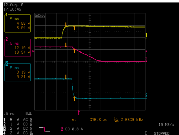
Figure 6: DS460S-3-002 Turn Off Characteristic via PS_ON Full Load: Vo = 36A, VSB = 2.3A Ch 1: PS_ON Ch 2: Vo Ch 3: PSOK
