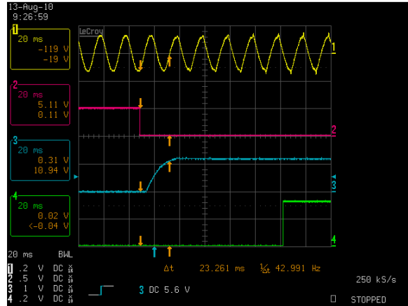
Figure 2: DS460S-3-002 Turn-on delay via PS_ON# – Vin = 90Vac Full Load: Vo = 36A, VSB = 2.3A Ch 1: AC Mains Ch 2: PS_ON# Ch 3: Vo Ch 4: PSOK
