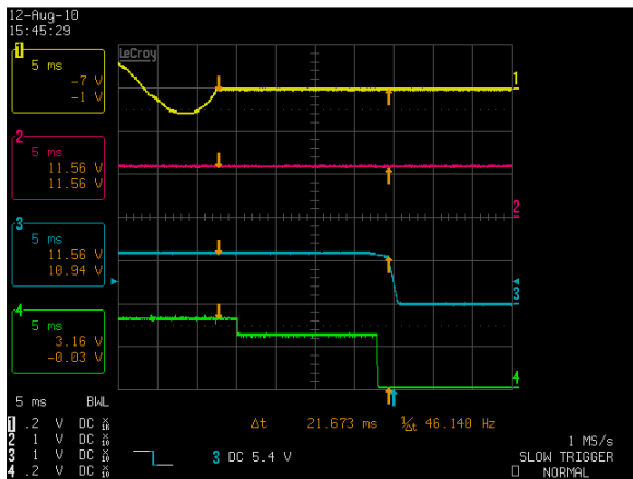
Figure 3: DS460S-3-002 Hold-up Time – Vin = 90Vac / 63Hz / 0° Full Load: Vo = 36A, VSB = 2.3A Ch 1: AC Mains Ch 2: VSB Ch 3: Vo Ch 4: PSOK
