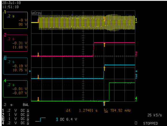
Figure 1: DS460S-3-002 Turn-on delay via AC mains – Vin = 90Vac Full Load: Vo = 36A, VSB = 2.3A Ch 1: AC Mains Ch 2: VSB Ch 3: Vo Ch 4: PSOK
