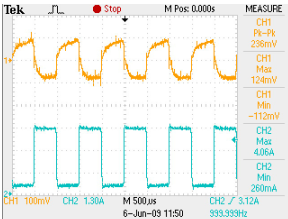
Figure 11: ADNB040-15-1PM-C Transient Response Vin = 230Vac Load: Io = 10% ~ 90% Duty: 1kHz Ch 1: Vo Ch 2: Iout
