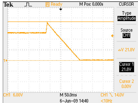
Figure 8: ADNB040-15-1PM-C Output Voltage Protection – Vin=88Vac Load: Io = 0.4A Ta = 25 °C Ch 1: Vo
