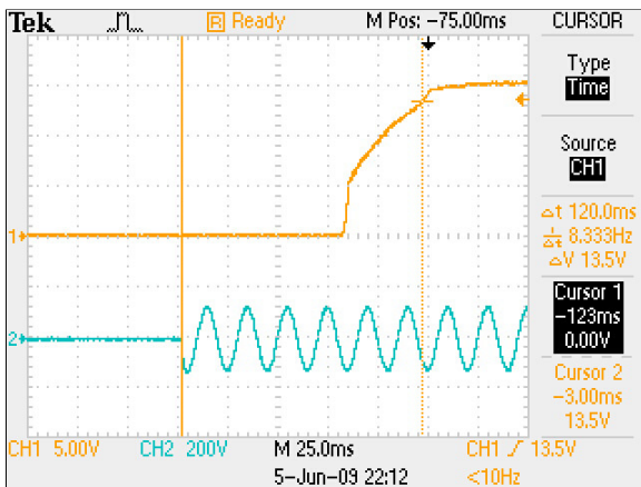
Figure 9: ADNB040-15-1PM-C Turn-on delay – Vin= 88Vac Load: Io = 4.0A Ta = 25 °C Ch 1: Vo Ch2:AC Mains
