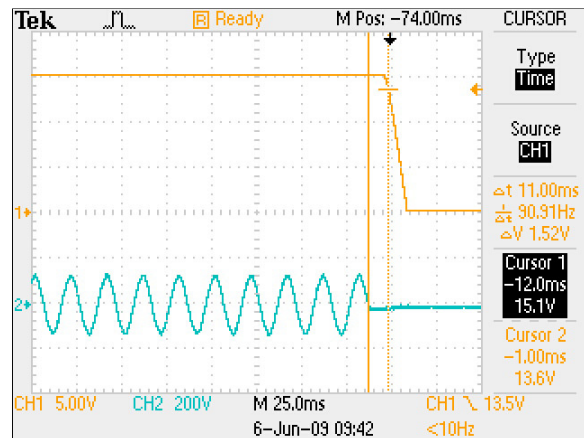
Figure 10: ADNB040-15-1PM-C Hold Up Time –Vin=88Vac Load: Io = 4.0A Ta = 25 °C Ch 1: Vo Ch 2: AC Mains
