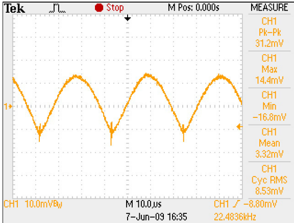
Figure 13: ADNB025-24-1PM-C Ripple and Noise Measurement – Vin = 88Vac Load: Io = 2.5A Ta = 25 °C Ch 1: Vo
