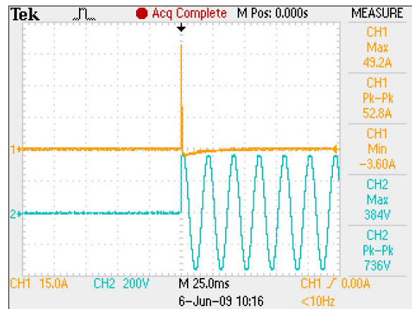
Figure 12: ADNB040-15-1PM-C Inrush Current Vin = 264Vac Load: Io = 4.0A Ta = 25 °C Ch 1: Iin Ch 2: AC Mains
