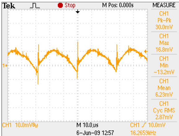
Figure 7: ADNB040-15-1PM-C Ripple and Noise Measurement – Vin = 88Vac Load: Io = 4.0A Ta = 25 °C Ch 1: Vo
