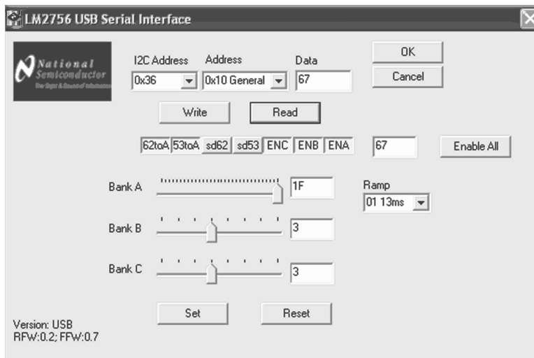
Figure 20. Example Configuration
