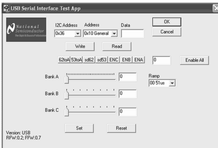
Figure 13. GUI Start-Up
