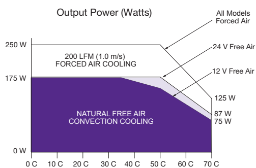
Figure 1: Derating Curve Output Power (Watts)
