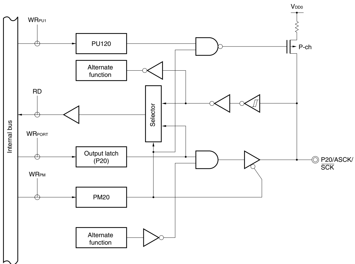
Figure 4-3. Block Diagram of P20
