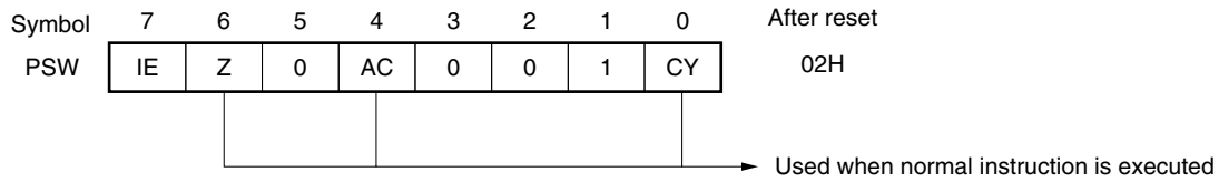
Figure 15-6. Configuration of Program Status Word
