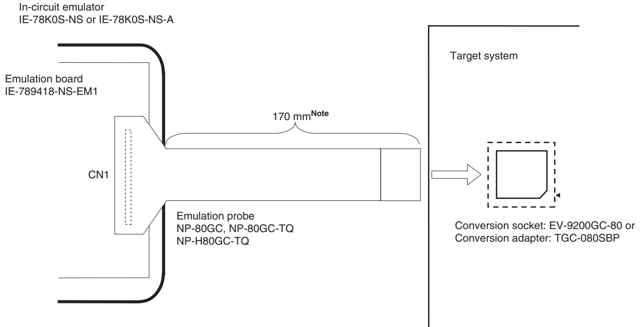
Figure B-1. Distance Between In-Circuit Emulator and Conversion Socket (80GC)
