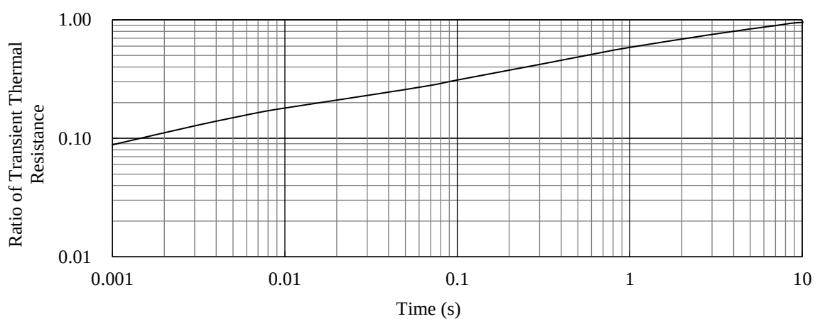
Figure 15-28. Transient Thermal Resistance: SIM6897M
