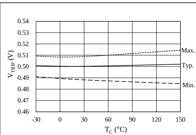
Figure 15-20. OCP Threshold Voltage, V_{TRIP} vs. T_C
