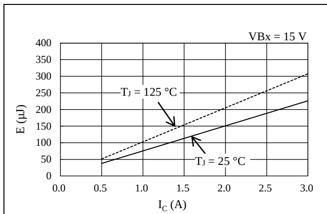
Figure 15-43. High-side Switching Loss
