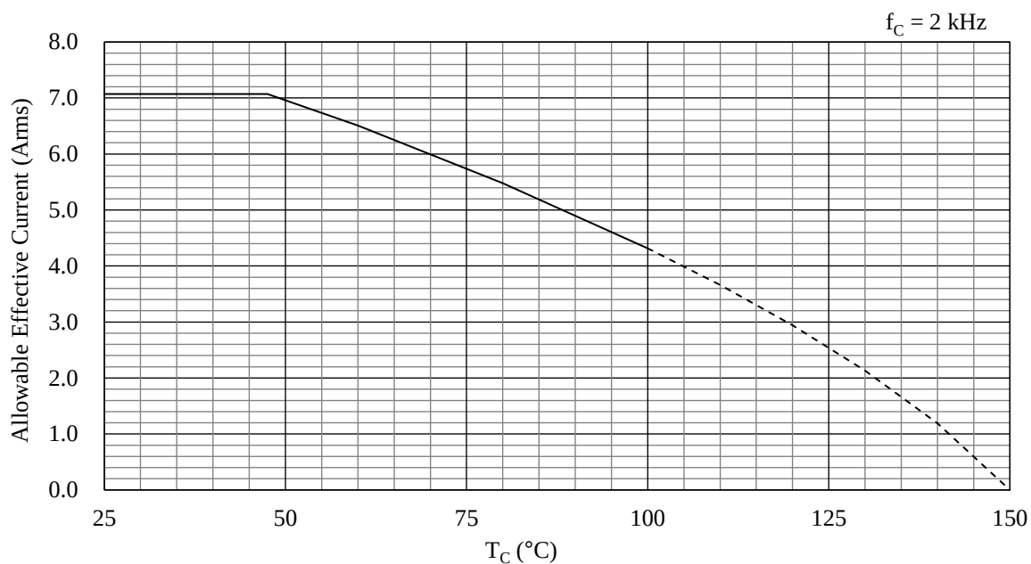
Figure 15-61. Allowable Effective Current ( f_C = 2 \text{ kHz} ): SIM6897M
