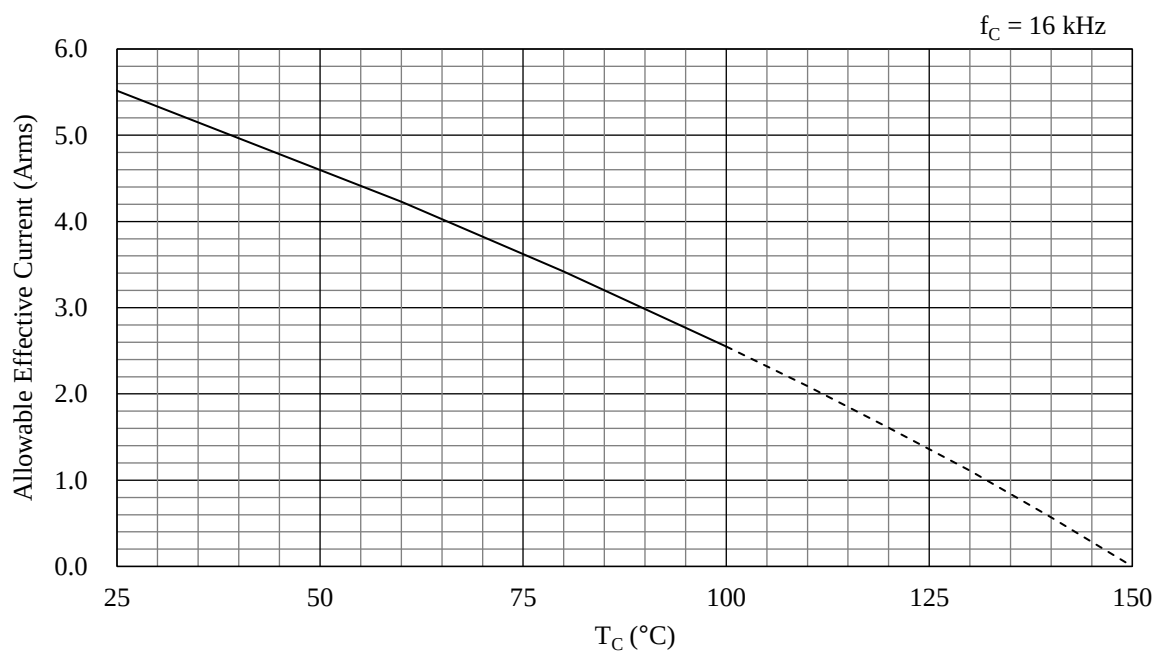
Figure 15-62. Allowable Effective Current ( f_C = 16 \text{ kHz} ): SIM6897M
