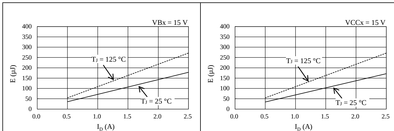
Figure 15-39. High-side Switching Loss
