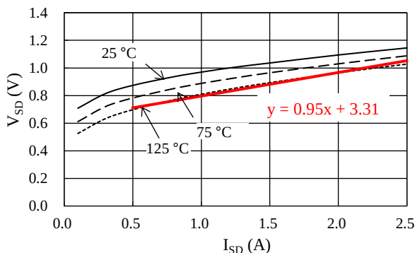
Figure 14-3. Linear Approximate Equation of V_{SD} vs. I_{SD}
