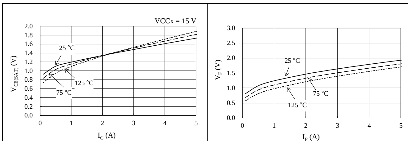
Figure 15-35. IGBT V_{CE(SAT)} vs. I_C
