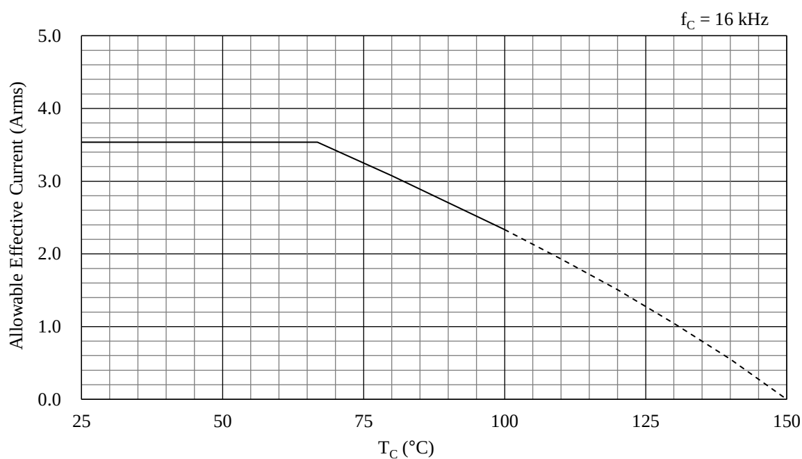
Figure 15-58. Allowable Effective Current ( f_C = 16 \text{ kHz} ): SIM6892M
