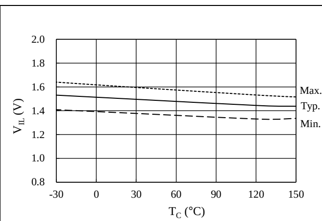
Figure 15-14. Low Level Input Threshold Voltage, V_{IL} vs. T_C
