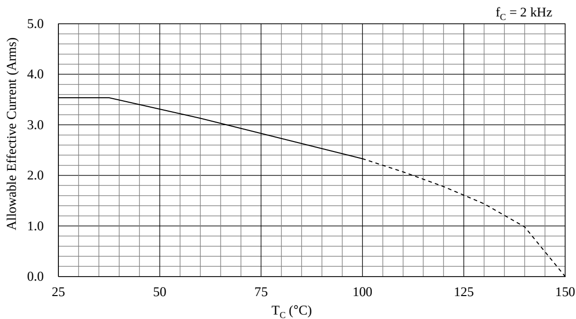
Figure 15-53. Allowable Effective Current ( f_C = 2 \text{ kHz} ): SIM6893M
