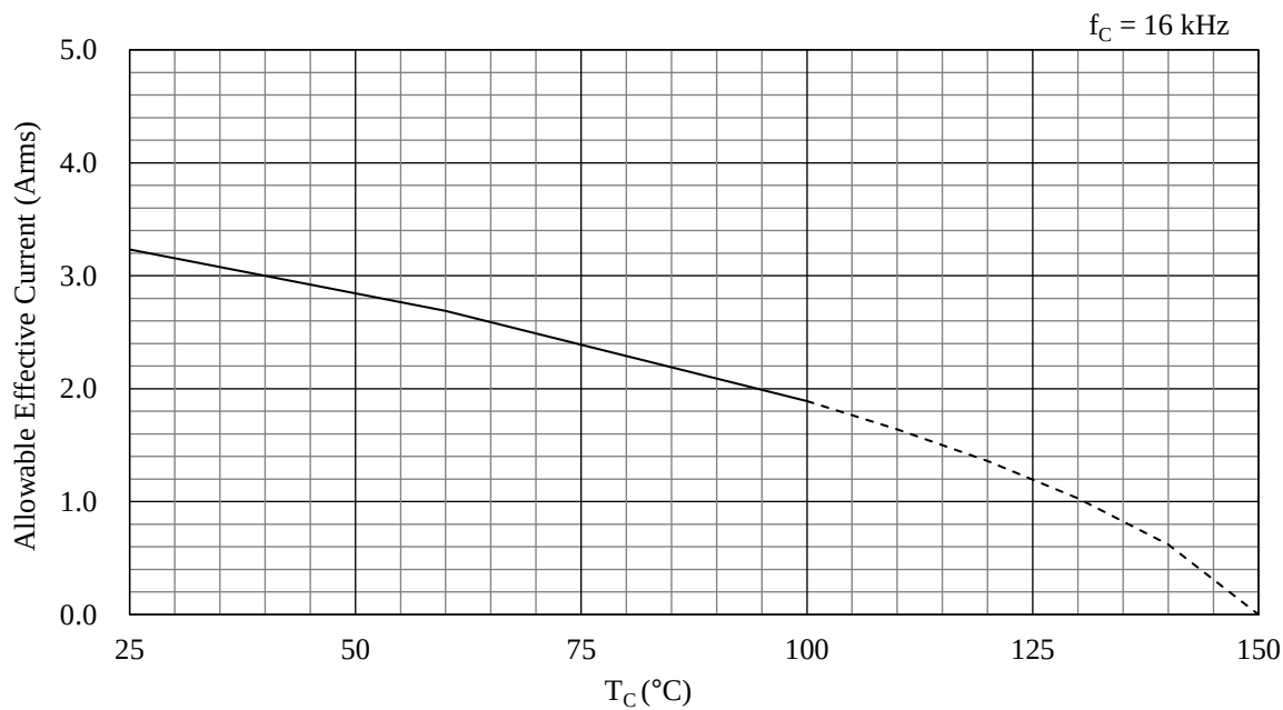
Figure 15-54. Allowable Effective Current ( f_C = 16 \text{ kHz} ): SIM6893M
