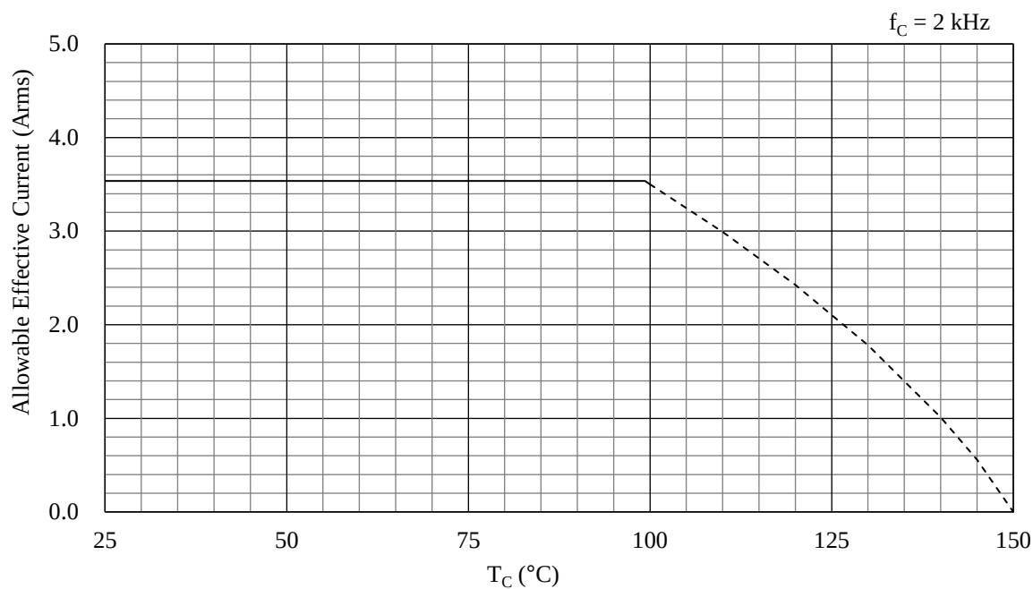
Figure 15-57. Allowable Effective Current ( f_C = 2 \text{ kHz} ): SIM6892M
