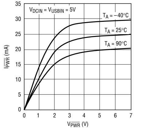
PWR Pin I-V Curve
