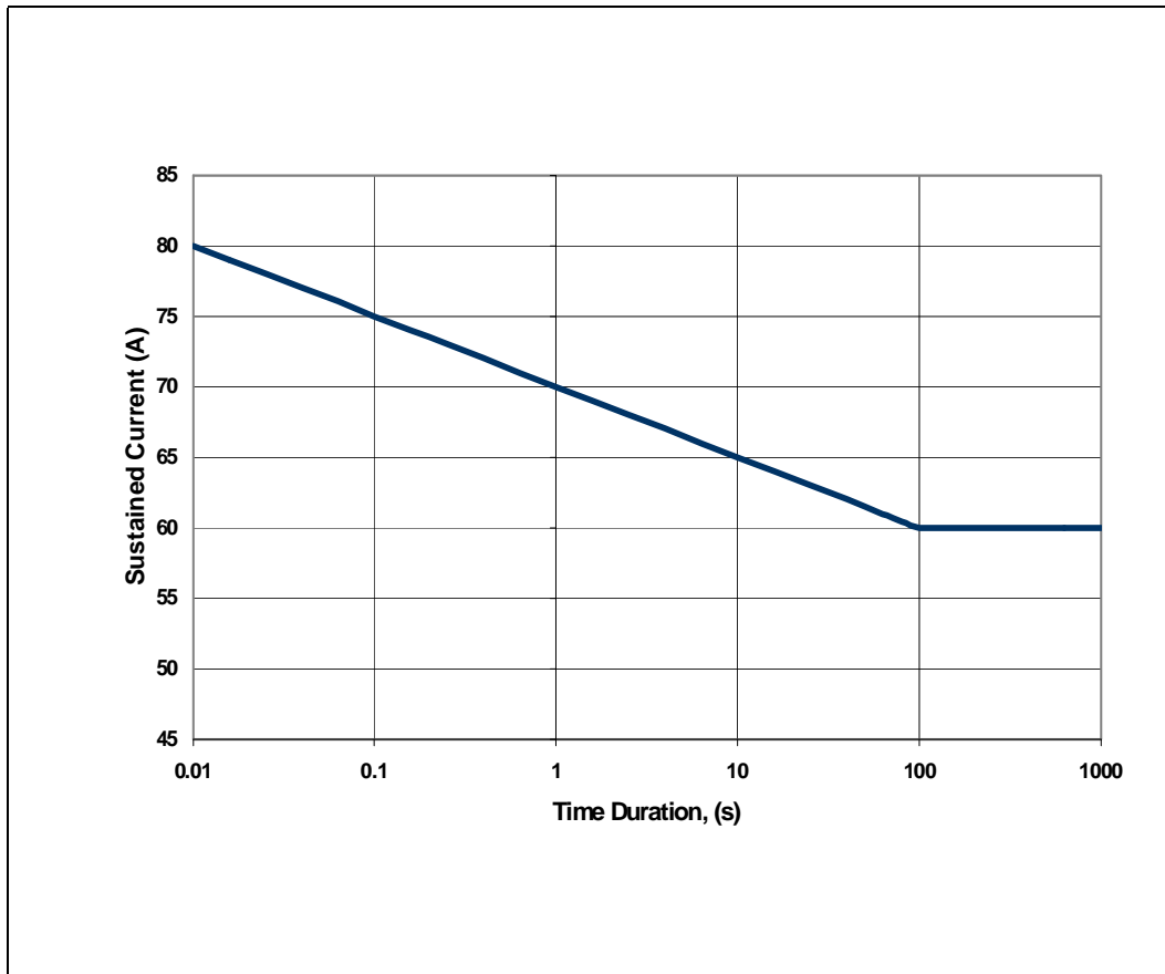
Figure 2-8. Load Current Versus Time (Low Power & LV-60W) 1,2
