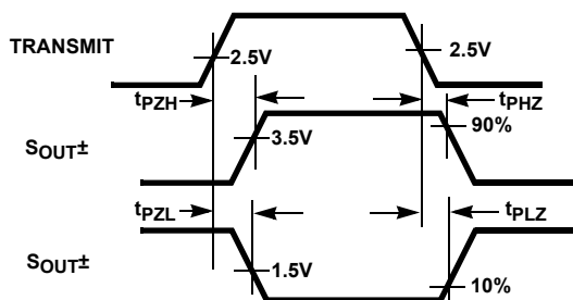
FIGURE 3B. MEASUREMENT POINTS
