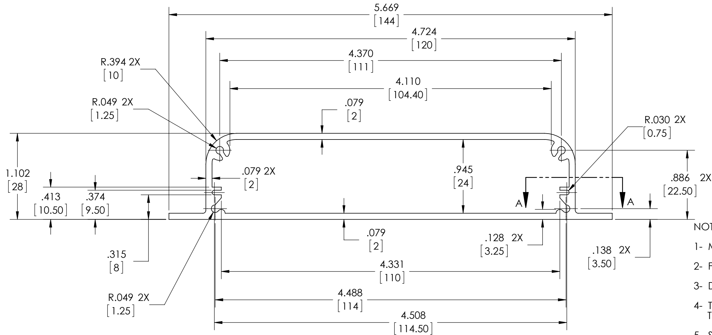
EXTRUSION PROFILE
