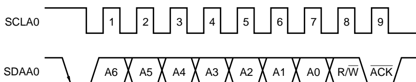
Figure 14-19. \overline{\text{ACK}}
