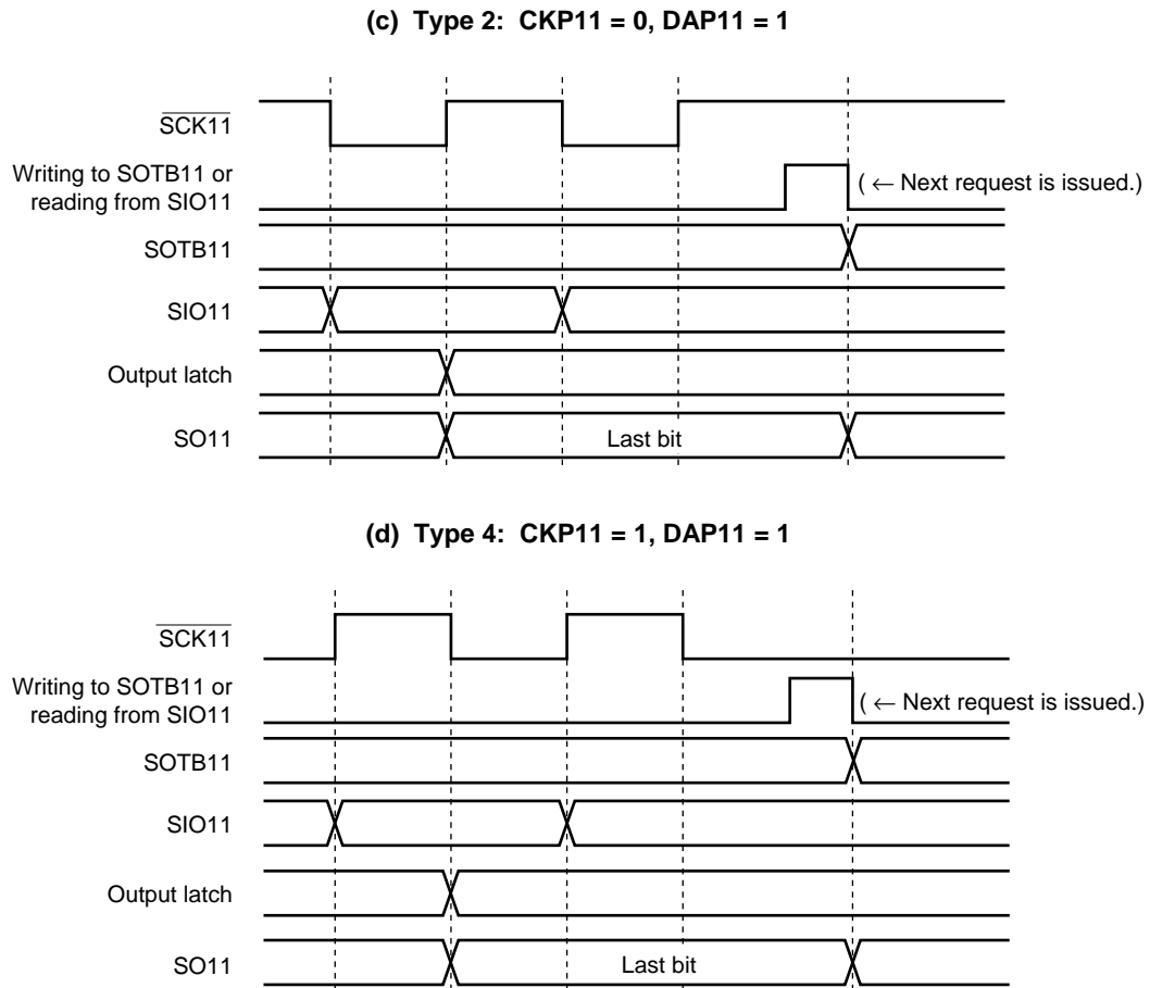
Figure 15-9. Output Value of SO11 Pin (Last Bit) (2/2)
