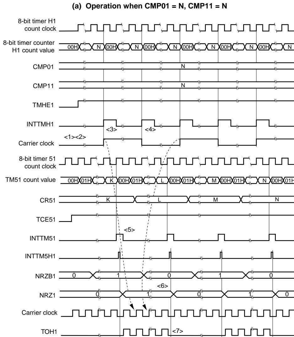
Figure 9-13. Carrier Generator Mode Operation Timing (1/3)
