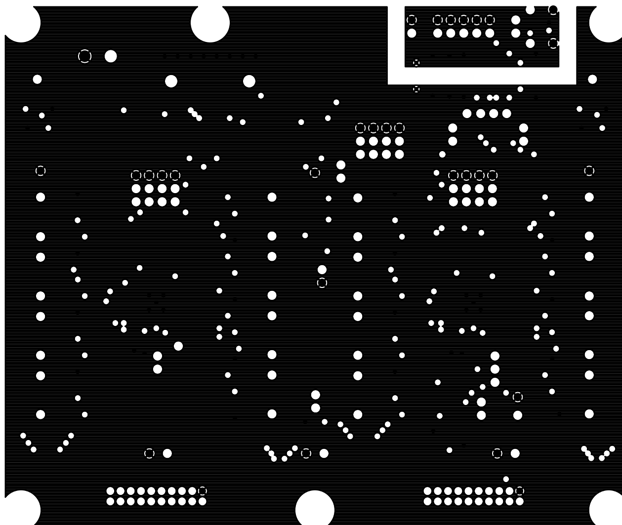
Figure 22. Evaluation Board Ground Layer
