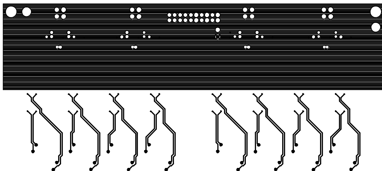
Figure 31. Connector Board Power Layer
