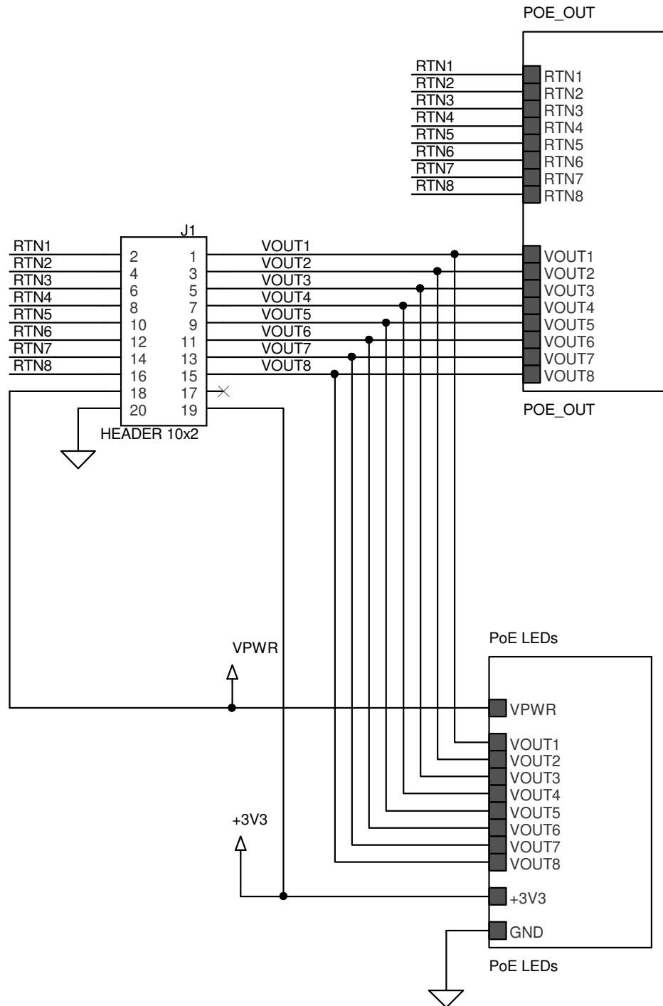
Figure 25. Connector Board Top Level
