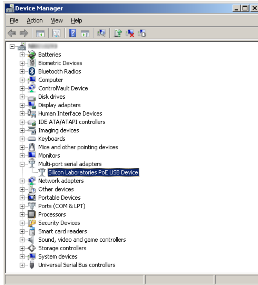
Figure 33. Device Manager
