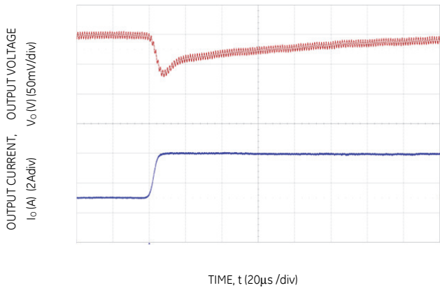
Figure 28 Transient Response to Dynamic Load Change from 50% to 100% at 12Vin, C out = 4x47uF, CTune=2700pF & RTune=300Ω
