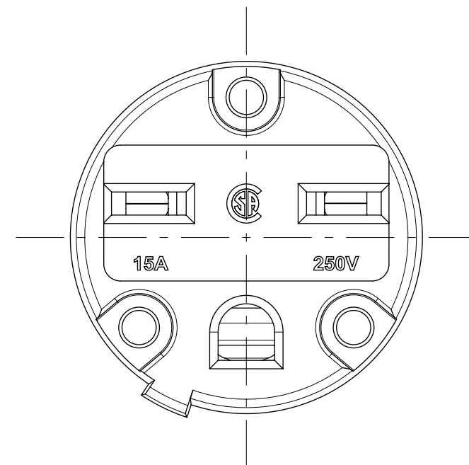
FACE VIEW
