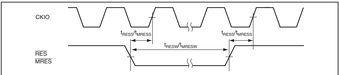
Figure 31.8 Reset Input Timing
