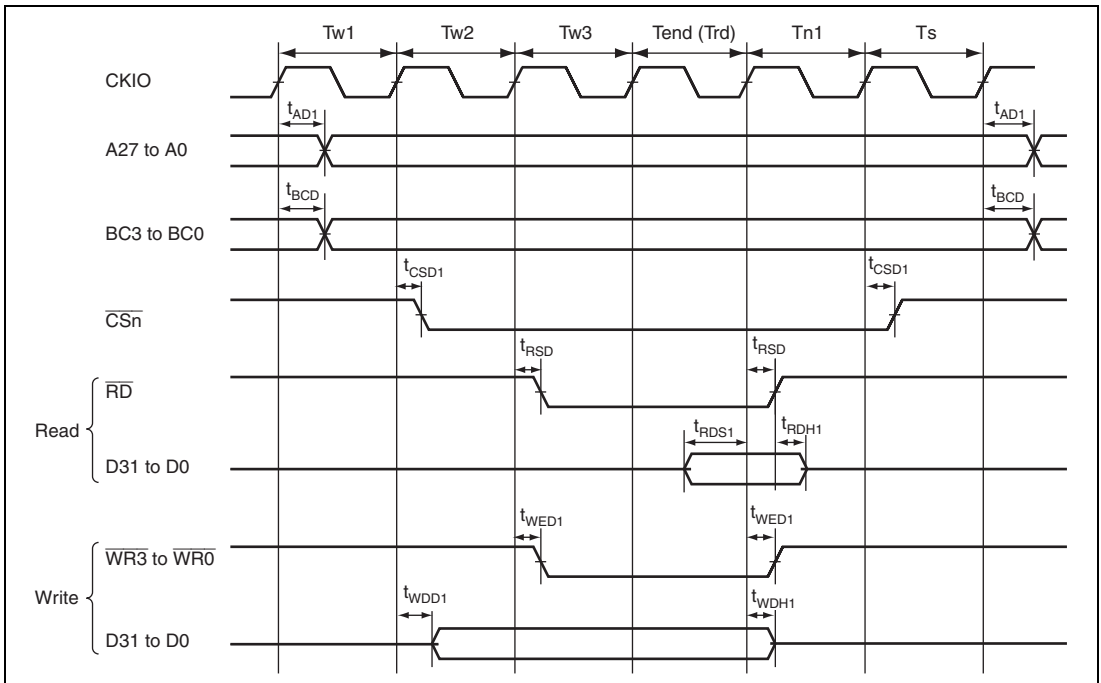
Figure 31.10 (1) External Address Space: Basic Bus Timing (Normal Access, Read/Write Cycle Wait = 3, CS Assert Wait = 1, Write Data Output Wait = 1, WR/RD Assert Wait = 2, Write Data Output Delay Cycles = 0, Read/Write CS Delay Cycles = 1)
