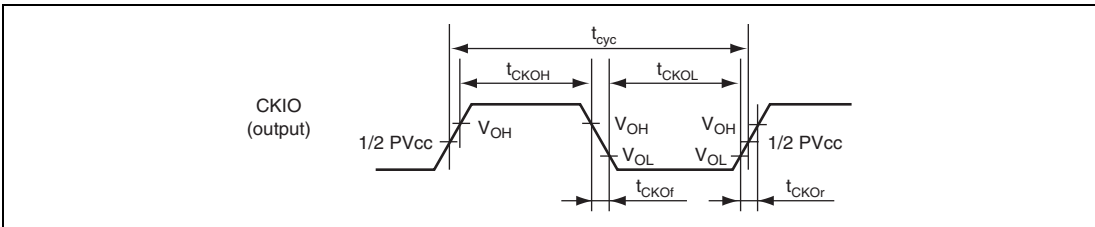
Figure 31.3 CKIO Clock Output Timing
