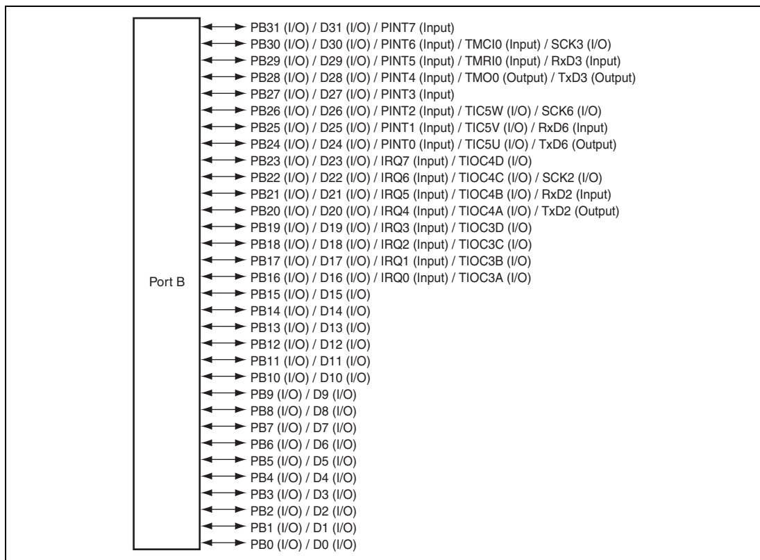
Figure 24.2 Port B
