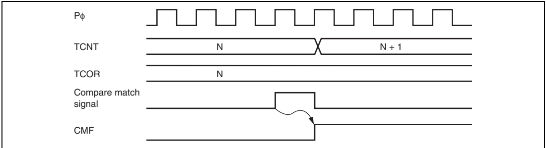
Figure 13.6 Timing of CMF Setting at Compare Match
