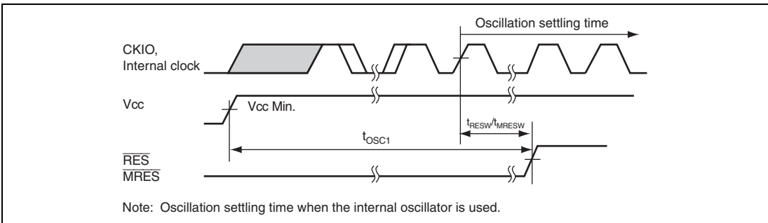
Figure 31.4 Power-On Oscillation Settling Time
