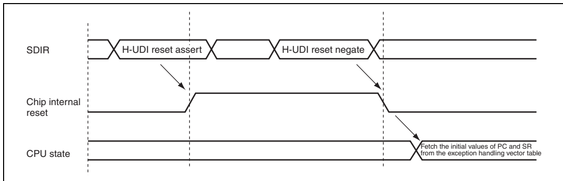
Figure 28.4 H-UDI Reset
