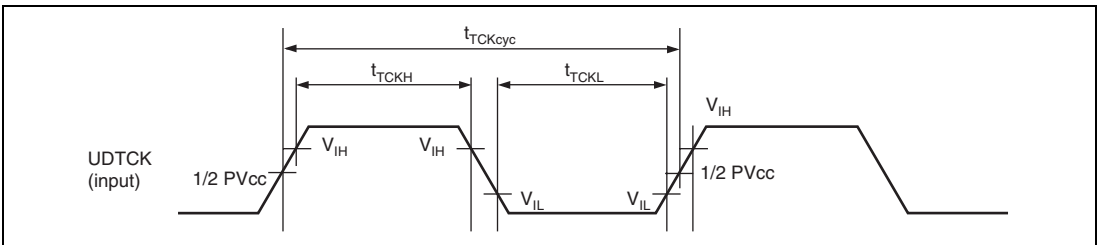
Figure 31.43 UDTCK Input Timing
