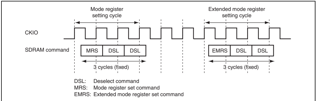
Figure 9.23 Operation Timing for Mode Register Setting
