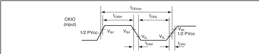
Figure 31.2 CKIO Clock Input Timing
