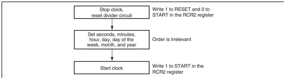
Figure 15.2 Setting Time
