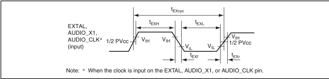
Figure 31.1 EXTAL, AUDIO_X1, and AUDIO_CLK Clock Input Timing
