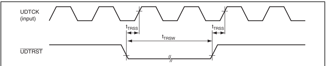
Figure 31.44 \overline{UDTRST} Input Timing
