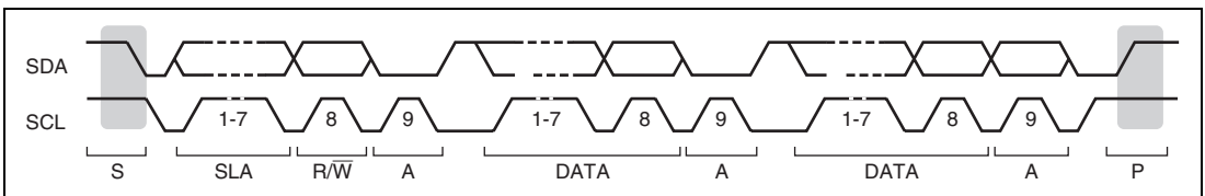
Figure 17.4 I 2 C Bus Timing
