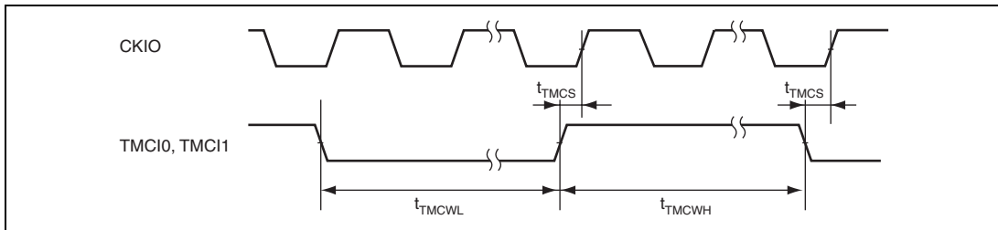
Figure 31.29 8-Bit Timer Clock Input Timing
