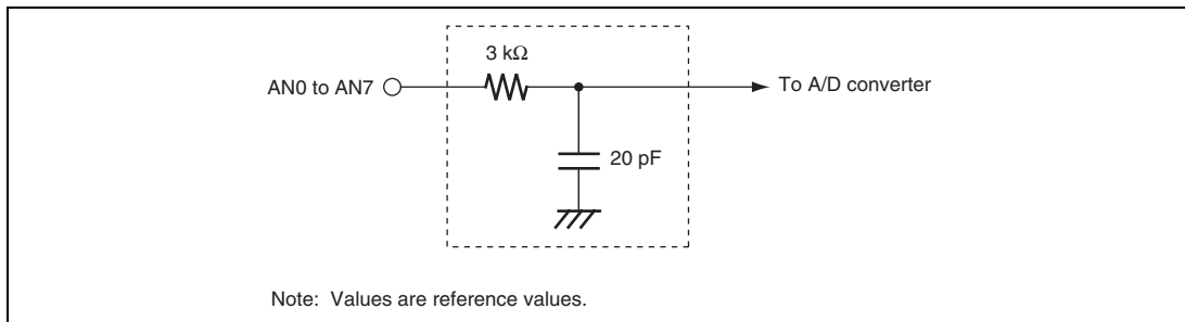
Figure 22.9 Analog Input Pin Equivalent Circuit
