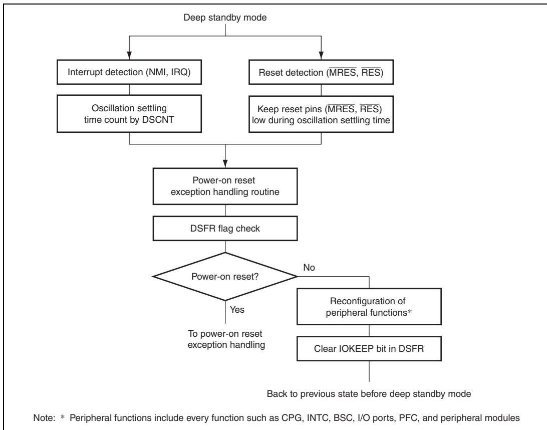
Figure 27.3 Flowchart of Canceling Deep Standby Mode
