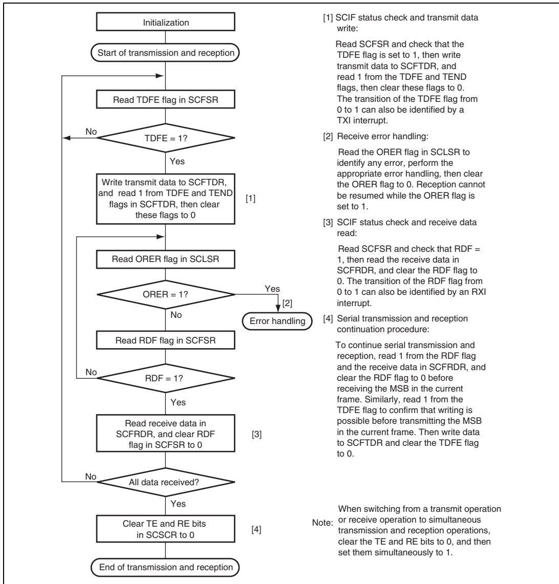
Figure 16.16 Sample Flowchart for Transmitting/Receiving Serial Data
