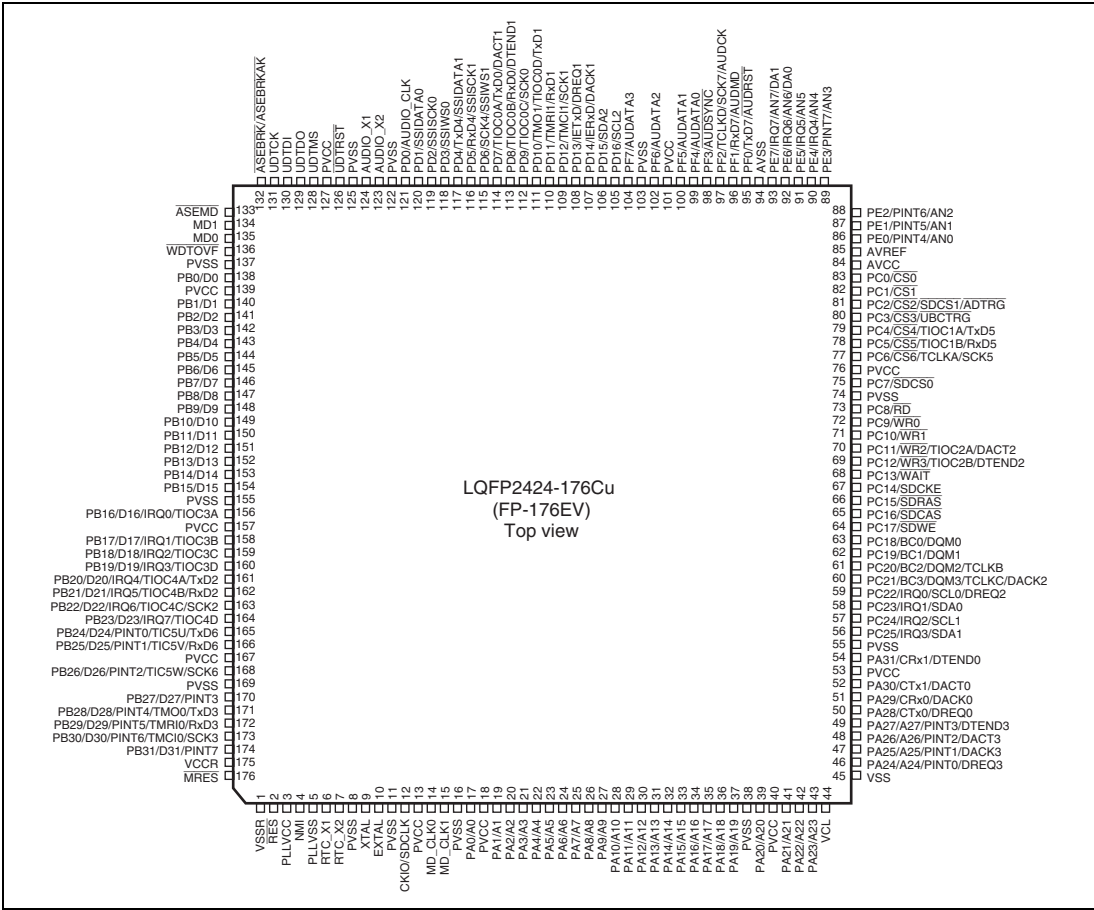
Figure 1.4 Pin Assignments of R5S72613
