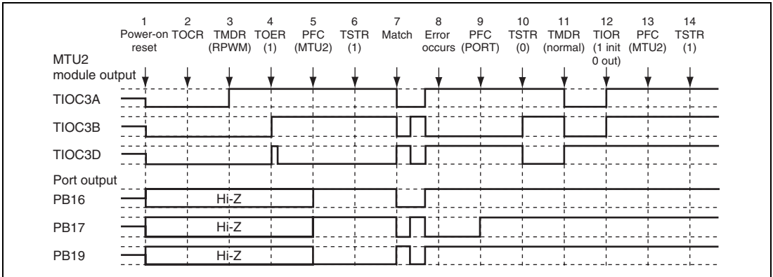
Figure 12.152 Error Occurrence in Reset-Synchronized PWM Mode, Recovery in Normal Mode
