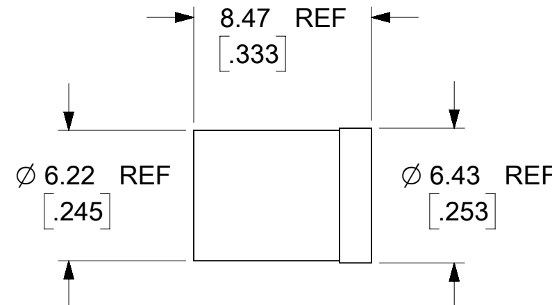
CRIMP TUBE
