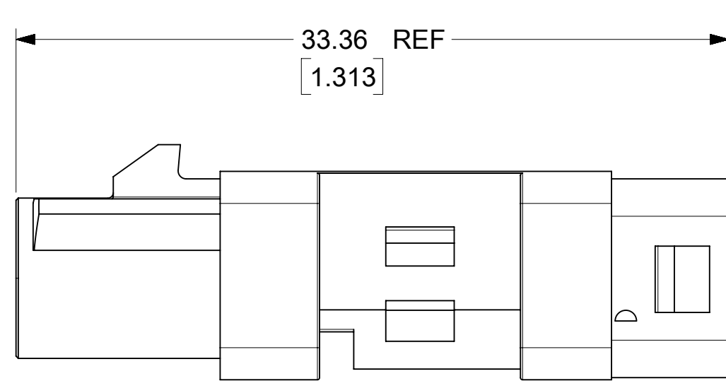
FAKRA JACK SHROUD (CODE E SHOWN)
