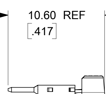
CONTACT (SHOWN LOOSE COMES T&R)
