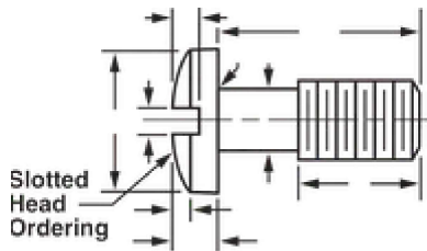
Slotted Head
