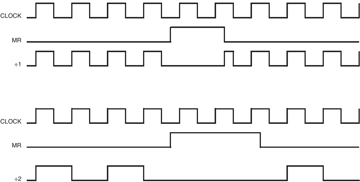
FIGURE 1. TIMING DIAGRAM
