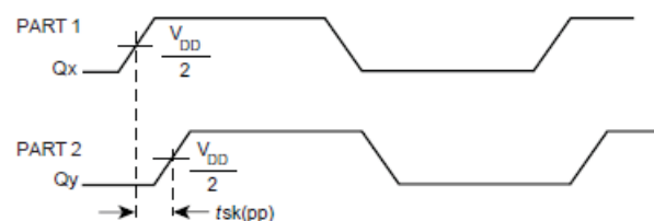
PART-TO-PART SKEW
