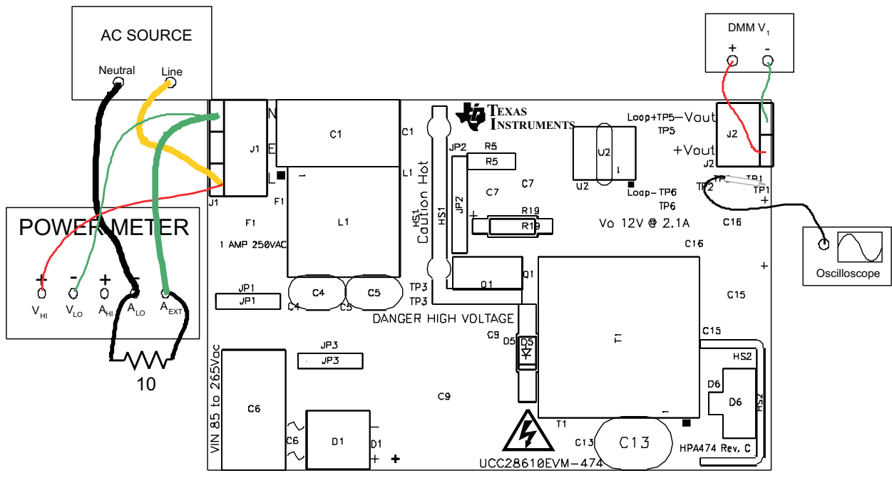
Figure 3. UCC28610EVM-474 Recommended Test Set Up Without a Load
