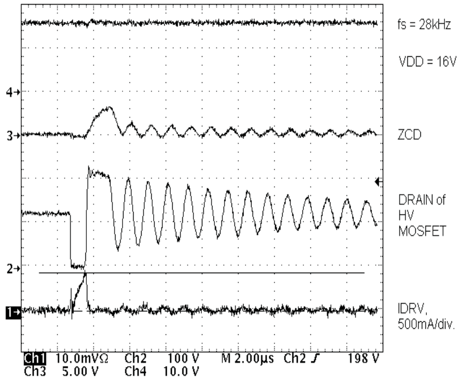
Figure 14. GM Mode Switching Cycle Waveform (Input voltage = 85 V AC , 0-A load, f_{SW} = 28\text{ kHz} , Ch.1 = I_{DRV} , 500 mA/div., I_{DRV} = 440\text{ mA} , Ch.2 = Drain of HV MOSFET, 100 V/div., Ch.3 = ZCD, 5 V/div., Ch. 4 = VDD, 10 V/div.)
