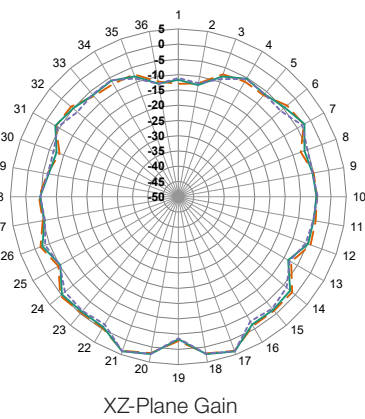
Figure 17. ANT-916-WRT Radiation Patterns, Center of Ground Plane
