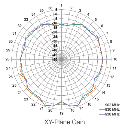
Figure 17. ANT-916-WRT Radiation Patterns, Center of Ground Plane
