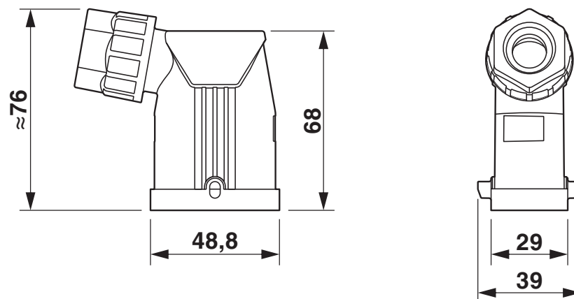
Dimensional drawing
