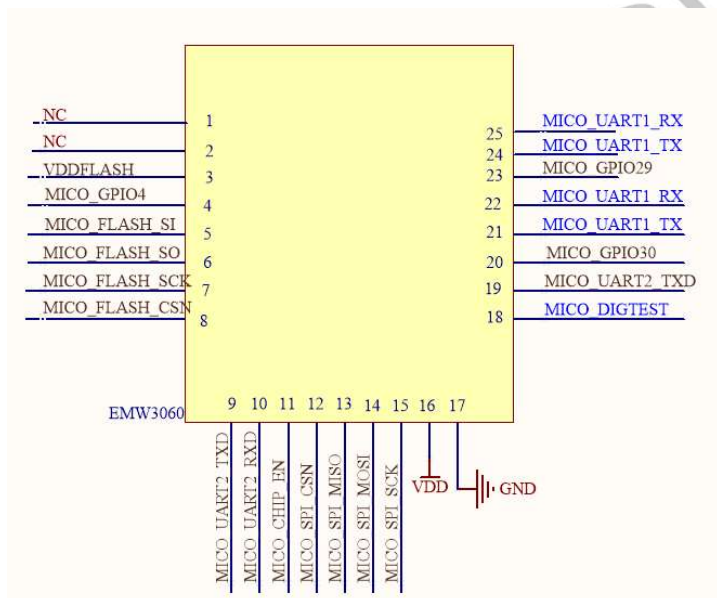
Figure 3 EMW3060 Package Definition
