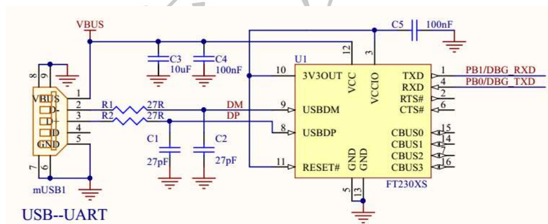
Figure 13 USB to UART
