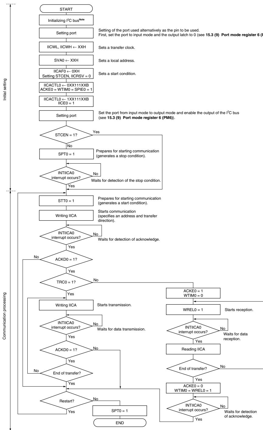
Figure 15-29. Master Operation in Single-Master System
