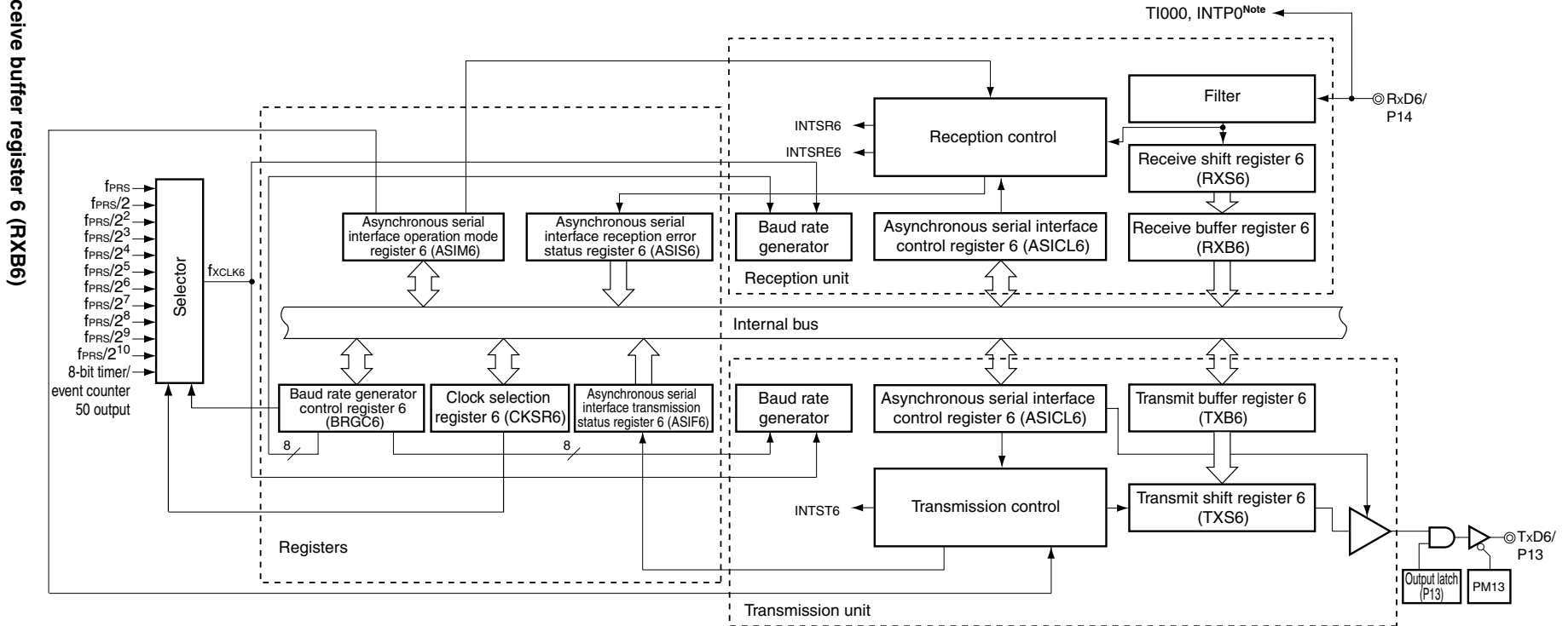
Figure 14-4. Block Diagram of Serial Interface UART6
