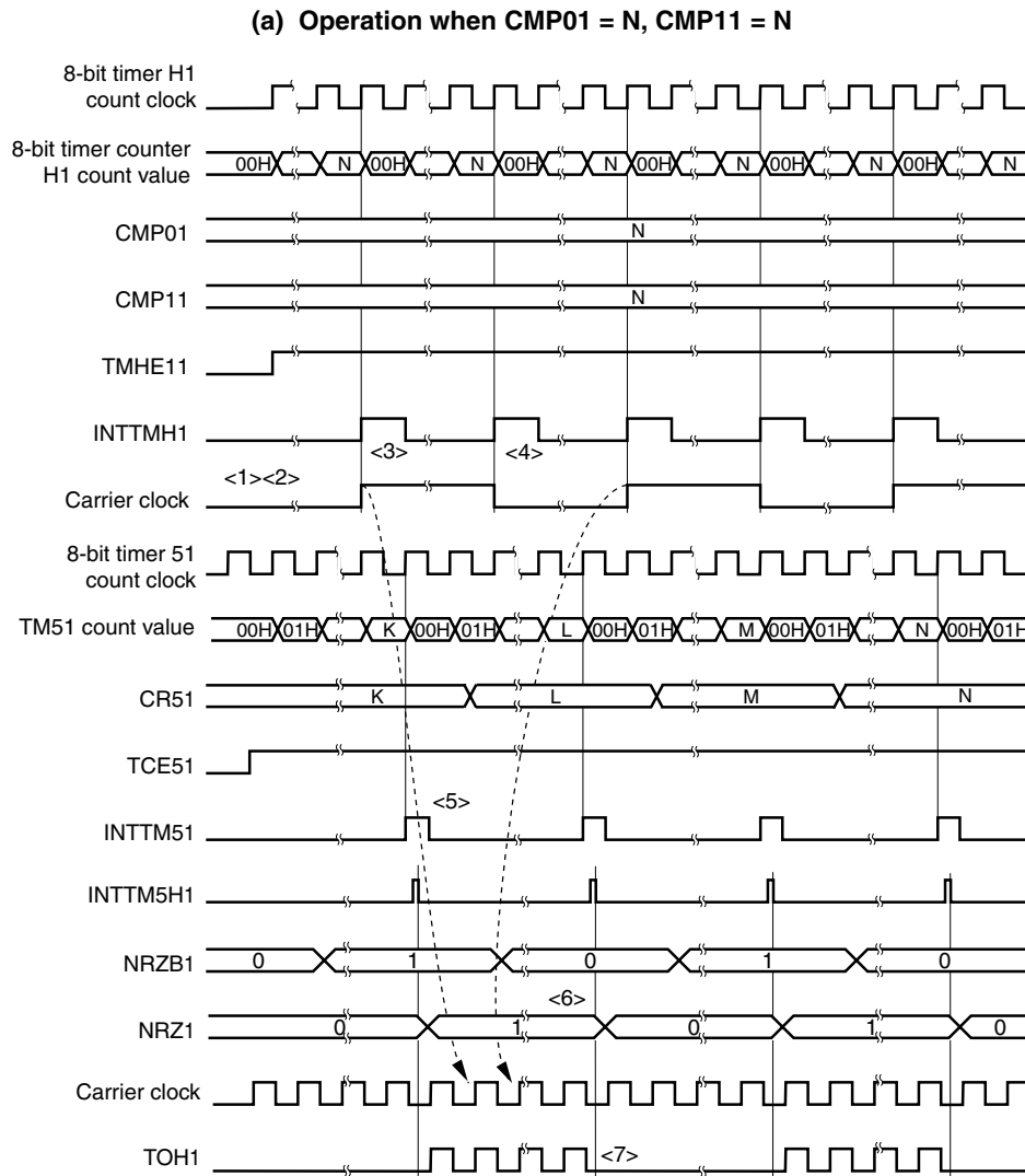
Figure 8-18. Carrier Generator Mode Operation Timing (1/3)
