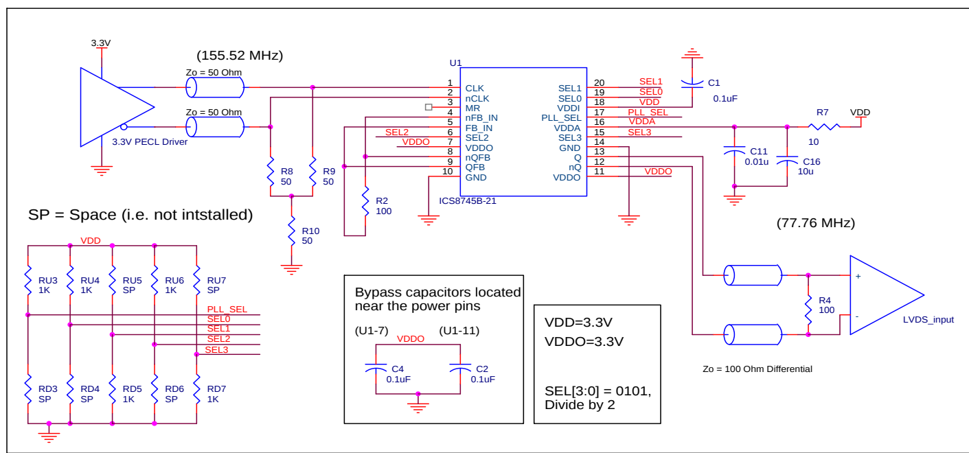
Figure 5A. 8745B-21 LVDS Zero Delay Buffer Schematic Example
