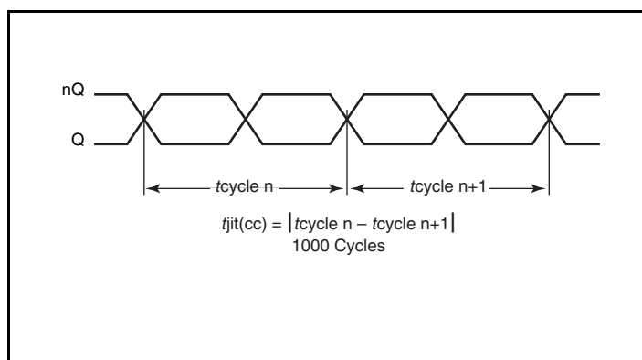
Cycle-to-Cycle Jitter
